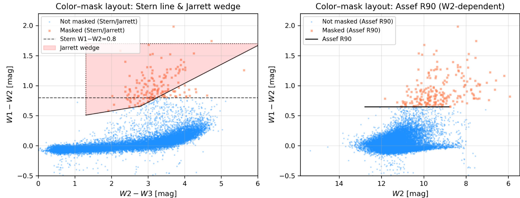
Figure 6. from Bo-Lun Huang et al 2026 Astron. J. 171 doi:10.3847/1538-3881/ae31e9 https://dx.doi.org/10.3847/1538-3881/ae31e9 © 2026. The Author(s). Published by the American Astronomical Society.
