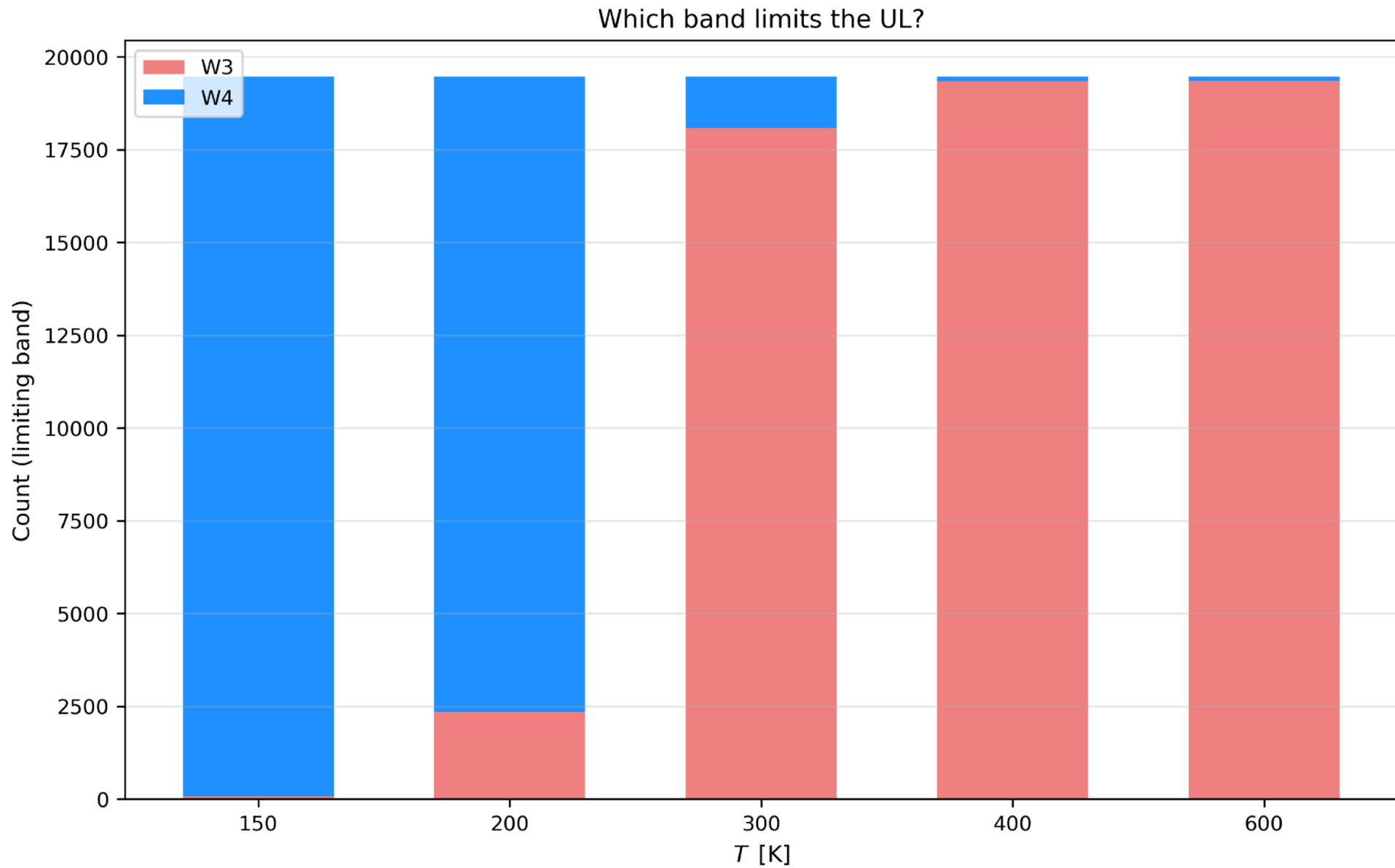
Figure 5. from Bo-Lun Huang et al 2026 Astron. J. 171 doi:10.3847/1538-3881/ae31e9 https://dx.doi.org/10.3847/1538-3881/ae31e9 © 2026. The Author(s). Published by the American Astronomical Society.
