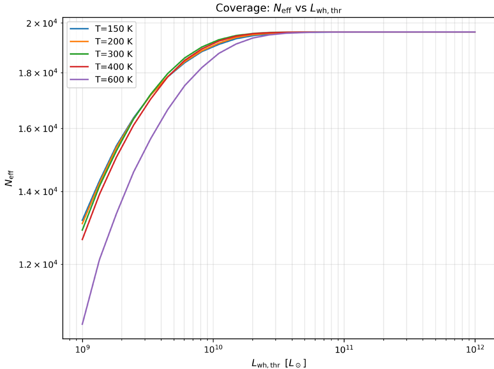
Figure 4. from Bo-Lun Huang et al 2026 Astron. J. 171 doi:10.3847/1538-3881/ae31e9 https://dx.doi.org/10.3847/1538-3881/ae31e9 © 2026. The Author(s). Published by the American Astronomical Society.
