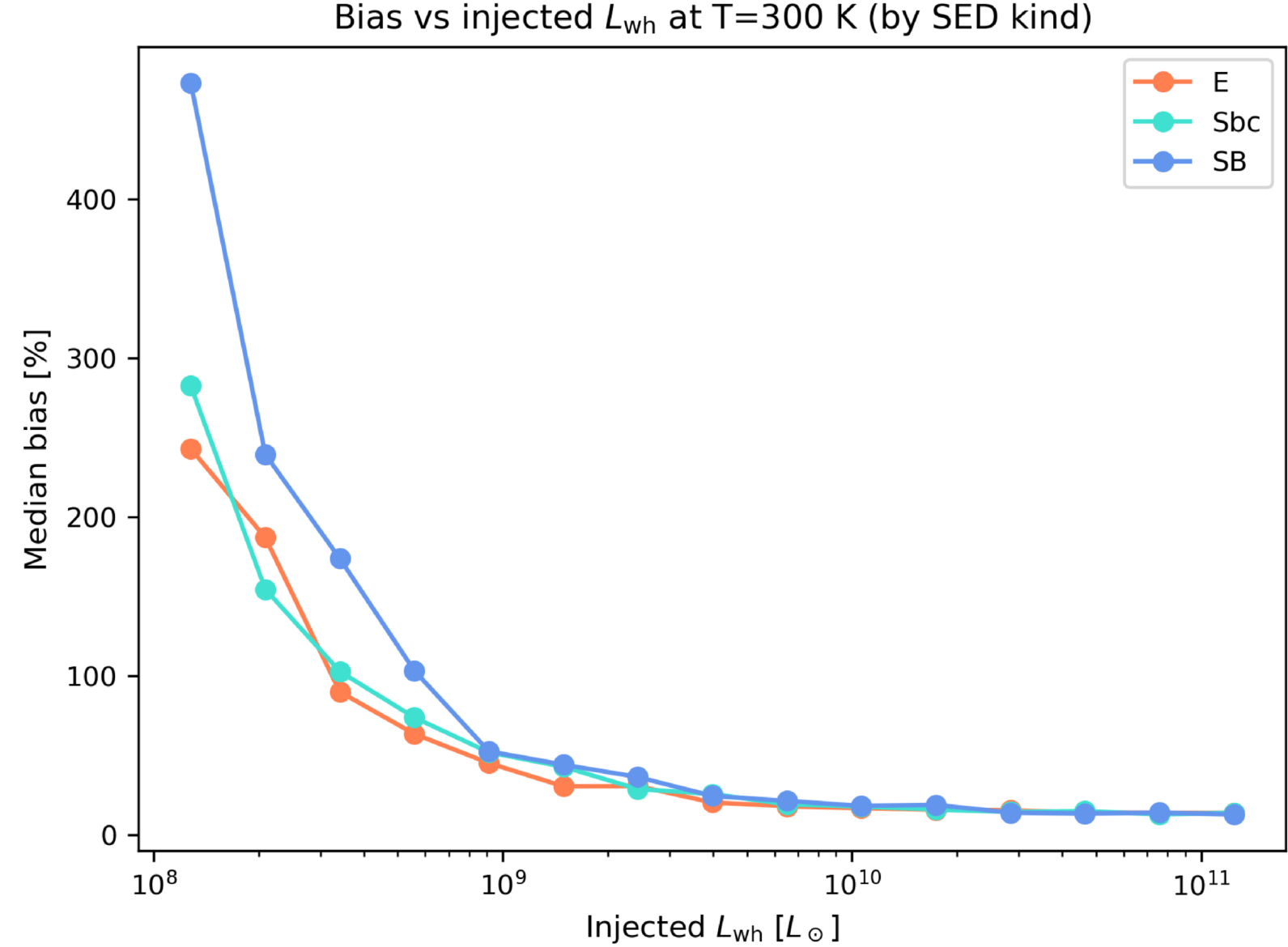
Figure 11. from Bo-Lun Huang et al 2026 Astron. J. 171 doi:10.3847/1538-3881/ae31e9 https://dx.doi.org/10.3847/1538-3881/ae31e9 © 2026. The Author(s). Published by the American Astronomical Society.
