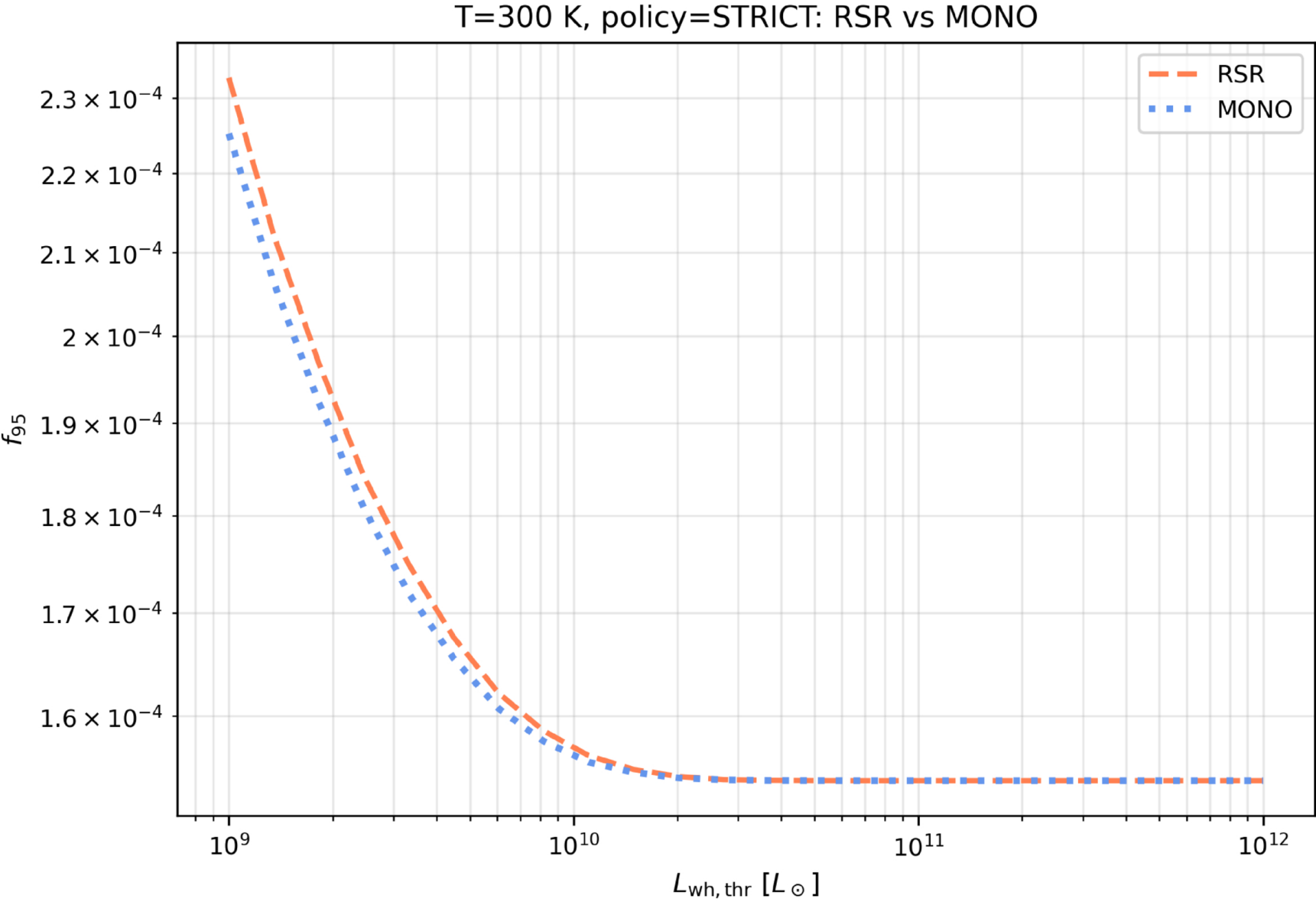
Figure 10. from Bo-Lun Huang et al 2026 Astron. J. 171 doi:10.3847/1538-3881/ae31e9 https://dx.doi.org/10.3847/1538-3881/ae31e9 © 2026. The Author(s). Published by the American Astronomical Society.
