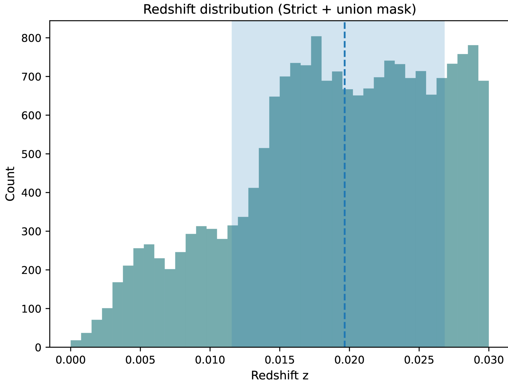
Figure 1. from Bo-Lun Huang et al 2026 Astron. J. 171 doi:10.3847/1538-3881/ae31e9 https://dx.doi.org/10.3847/1538-3881/ae31e9 © 2026. The Author(s). Published by the American Astronomical Society.
