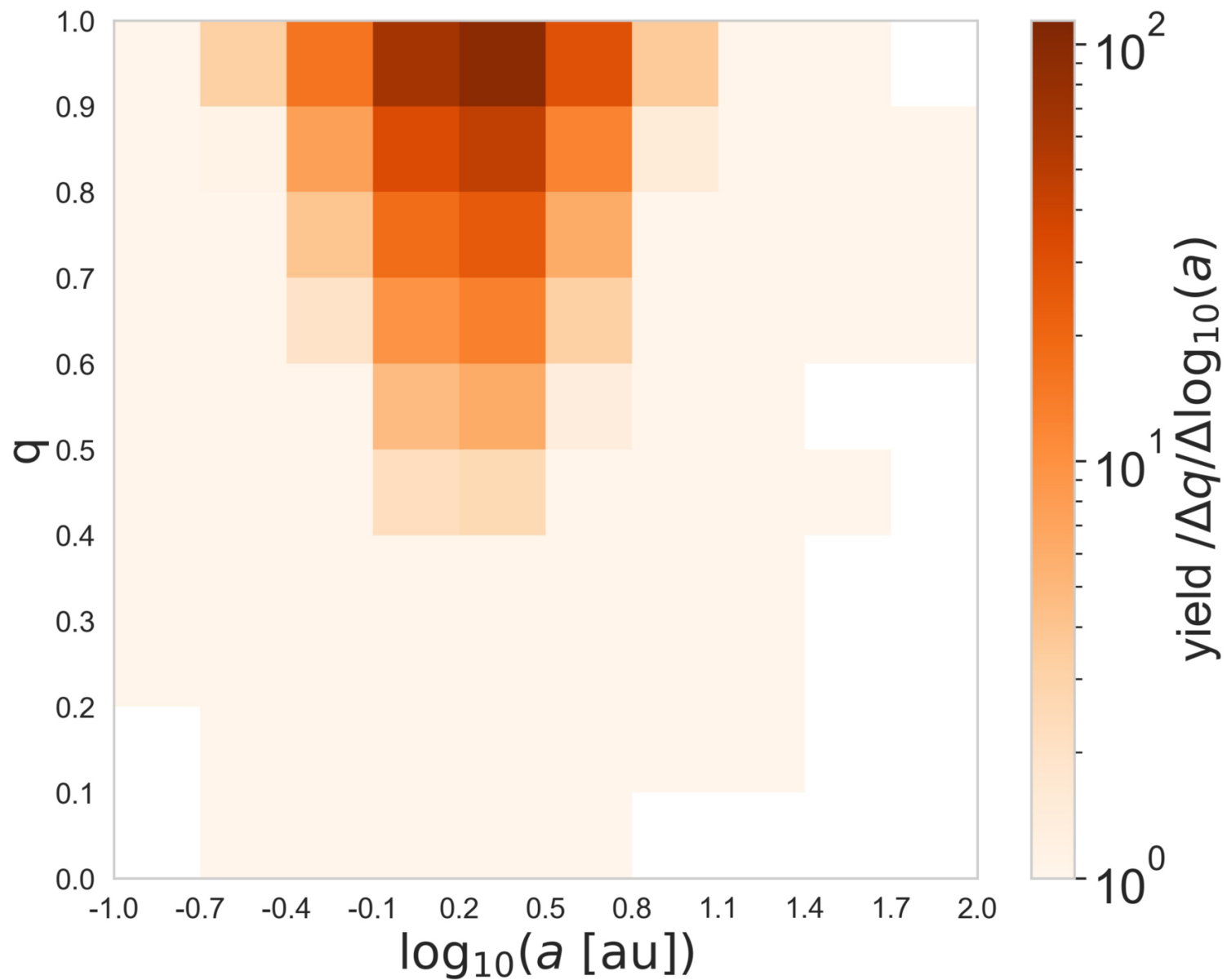
Figure 6. from Yifan Xuan et al 2026 Astron. J. 171 doi:10.3847/1538-3881/ae3176 https://dx.doi.org/10.3847/1538-3881/ae3176 © 2026. The Author(s). Published by the American Astronomical Society.
