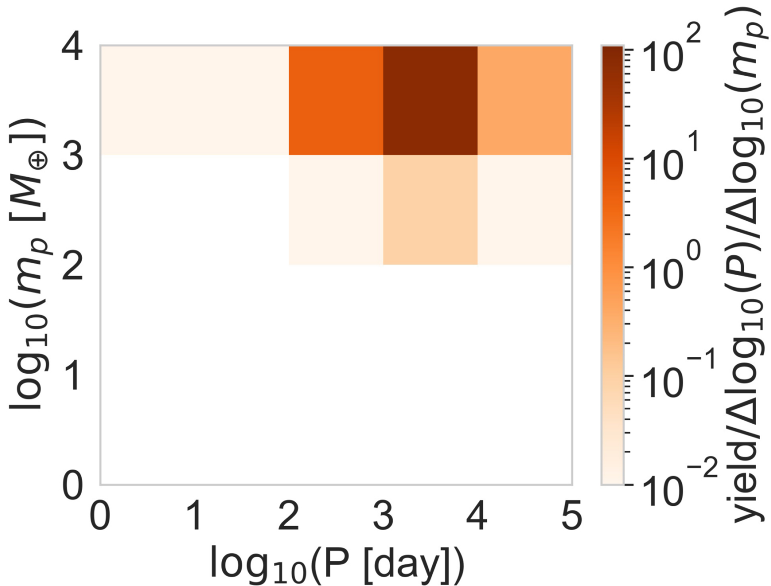
Figure 5. from Yifan Xuan et al 2026 Astron. J. 171 doi:10.3847/1538-3881/ae3176 https://dx.doi.org/10.3847/1538-3881/ae3176 © 2026. The Author(s). Published by the American Astronomical Society.
