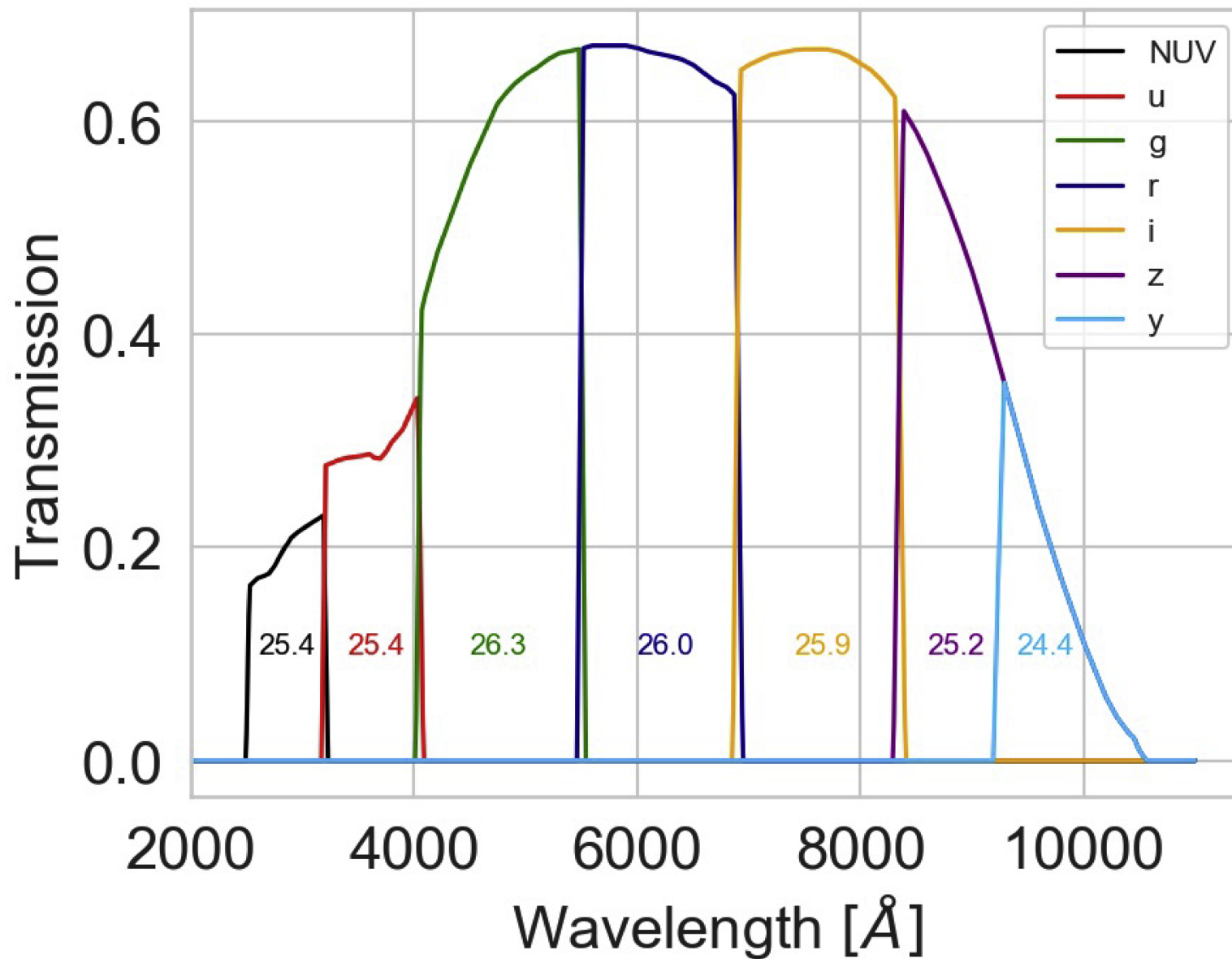
Figure 4. from Yifan Xuan et al 2026 Astron. J. 171 doi:10.3847/1538-3881/ae3176 https://dx.doi.org/10.3847/1538-3881/ae3176 © 2026. The Author(s). Published by the American Astronomical Society.
