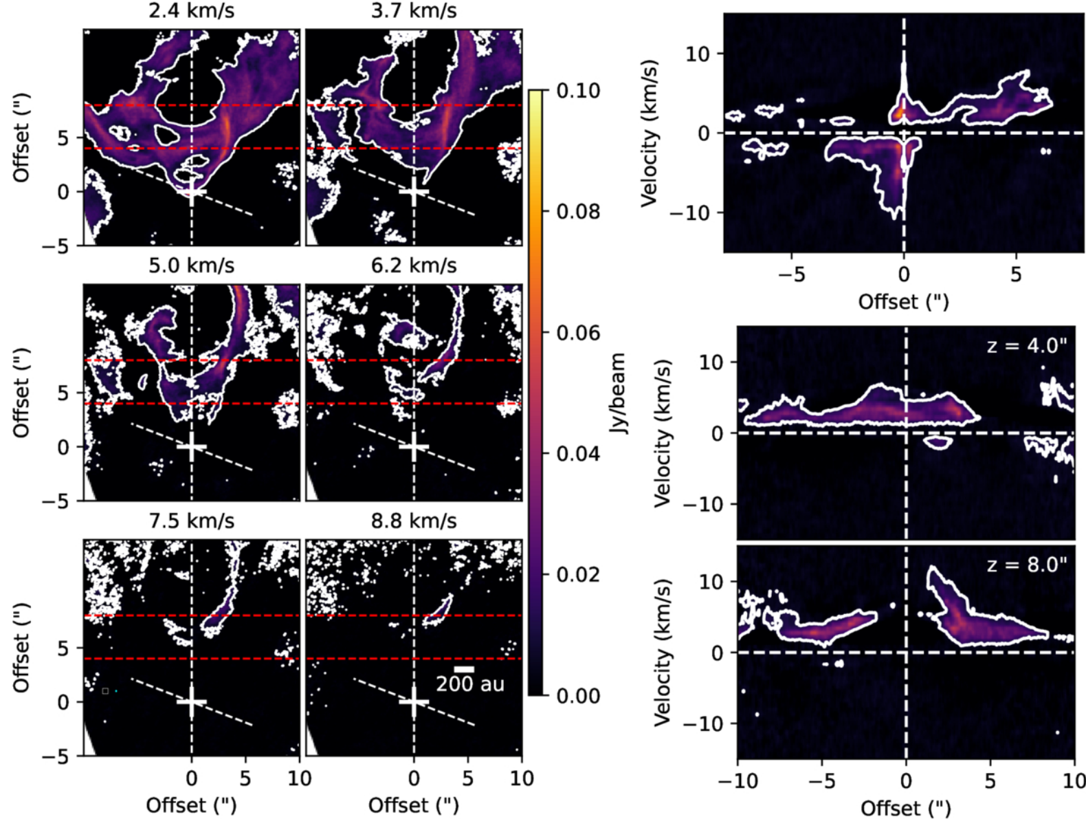
Figure 7. from Anton Feeney-Johansson et al 2026 Astron. J. 171 doi:10.3847/1538-3881/ae3135 https://dx.doi.org/10.3847/1538-3881/ae3135 © 2026. The Author(s). Published by the American Astronomical Society.
