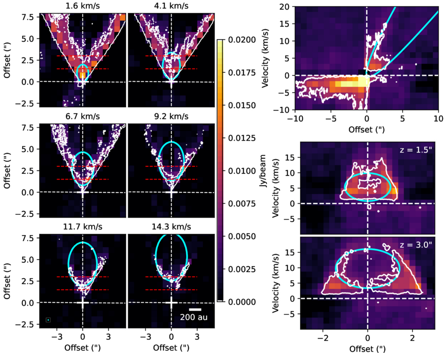
Figure 6. from Anton Feeney-Johansson et al 2026 Astron. J. 171 doi:10.3847/1538-3881/ae3135 https://dx.doi.org/10.3847/1538-3881/ae3135 © 2026. The Author(s). Published by the American Astronomical Society.
