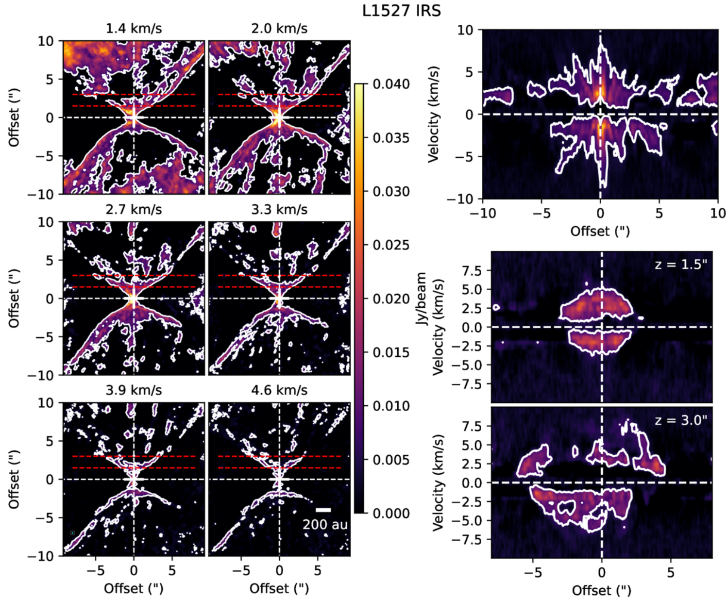
Figure 5. from Anton Feeney-Johansson et al 2026 Astron. J. 171 doi:10.3847/1538-3881/ae3135 https://dx.doi.org/10.3847/1538-3881/ae3135 © 2026. The Author(s). Published by the American Astronomical Society.
