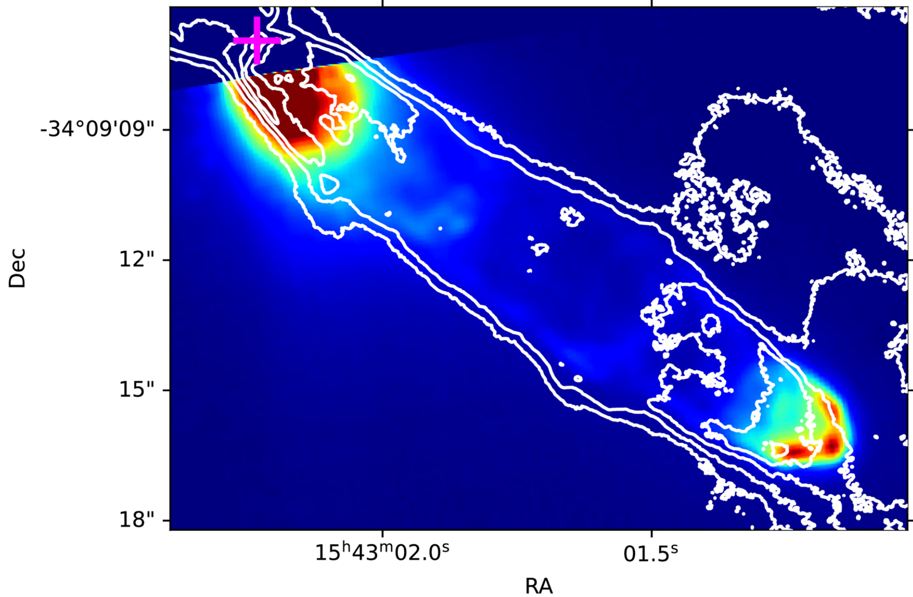
Figure 3. from Anton Feeney-Johansson et al 2026 Astron. J. 171 doi:10.3847/1538-3881/ae3135 https://dx.doi.org/10.3847/1538-3881/ae3135 © 2026. The Author(s). Published by the American Astronomical Society.
