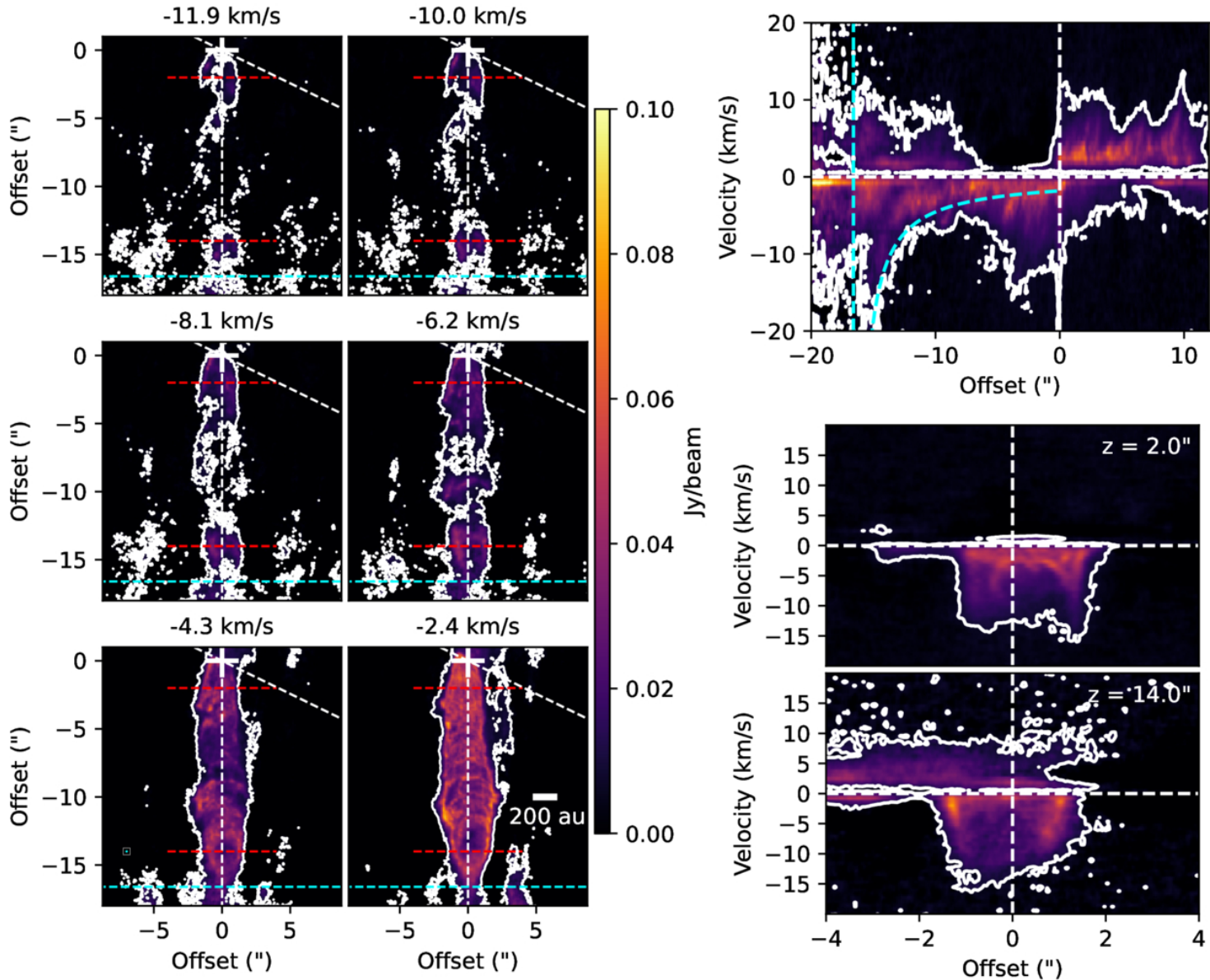
Figure 2. from Anton Feeney-Johansson et al 2026 Astron. J. 171 doi:10.3847/1538-3881/ae3135 https://dx.doi.org/10.3847/1538-3881/ae3135 © 2026. The Author(s). Published by the American Astronomical Society.
