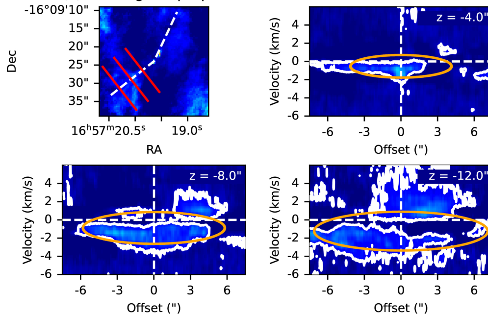
(c) P–V diagram perpendicular to the outflow axis
