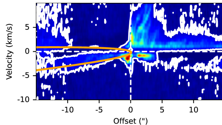
(c) P–V diagram perpendicular to the outflow axis
