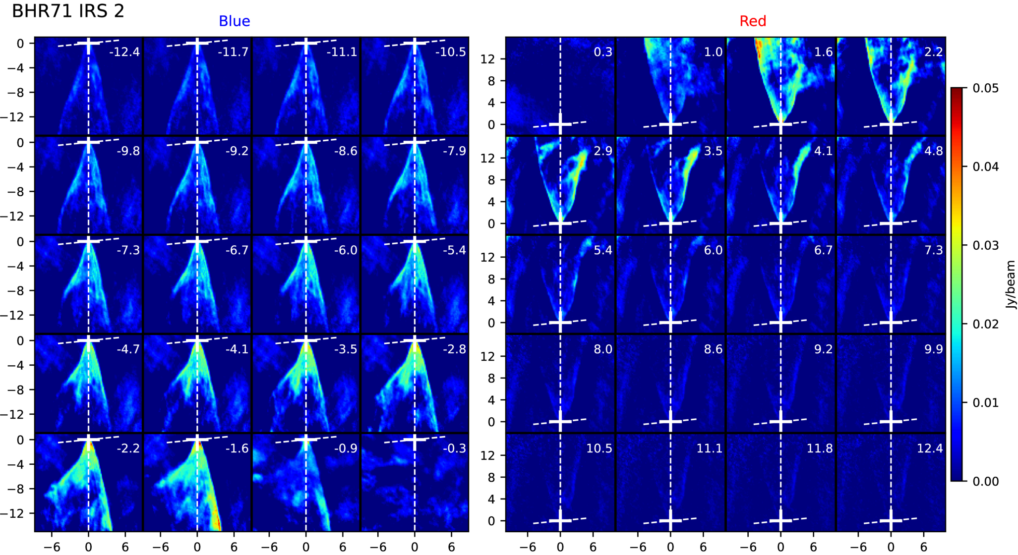
Figure 10. Channel maps from Anton Feeney-Johansson et al 2026 Astron. J. 171 doi:10.3847/1538-3881/ae3135 https://dx.doi.org/10.3847/1538-3881/ae3135 © 2026. The Author(s). Published by the American Astronomical Society.
