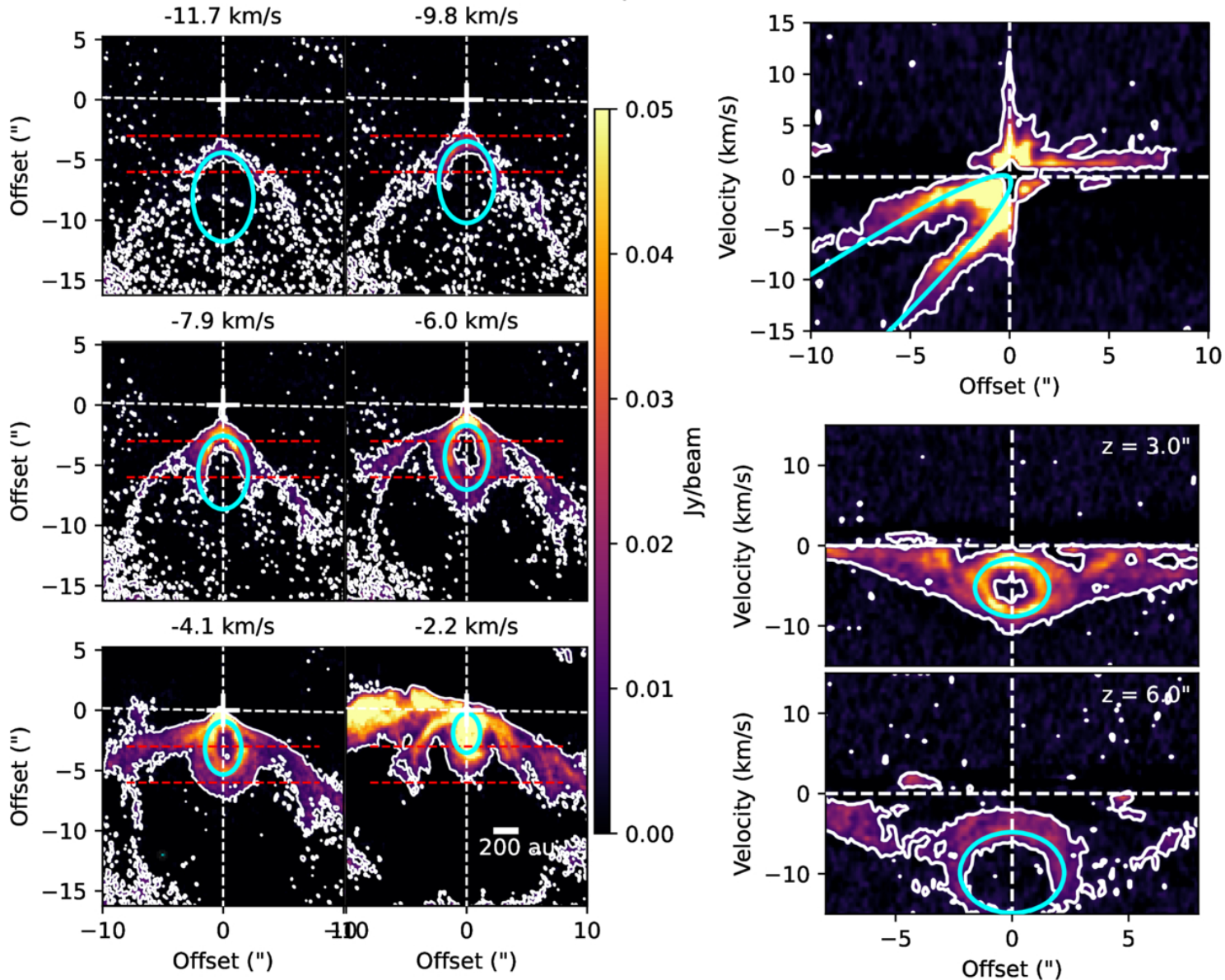
Figure 1. from Anton Feeney-Johansson et al 2026 Astron. J. 171 doi:10.3847/1538-3881/ae3135 https://dx.doi.org/10.3847/1538-3881/ae3135 © 2026. The Author(s). Published by the American Astronomical Society.
