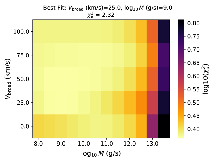
(c) All species, T_{\text{iso}}=8,000 K
