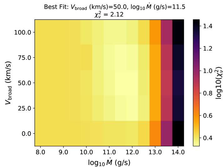
(a) All species, T_{\text{input}}=13,200 K
