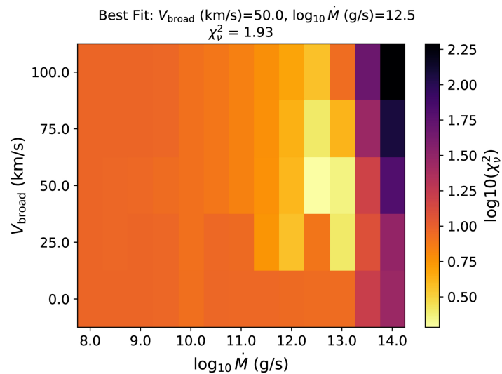
(b) Mg II only, T_{\text{input}}=13,200 K
