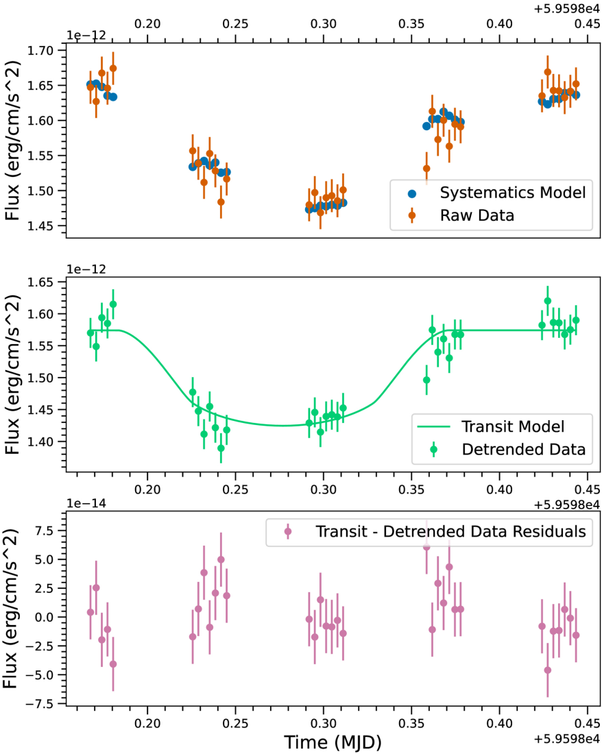
Inside Mg II (2802.4 Å)
