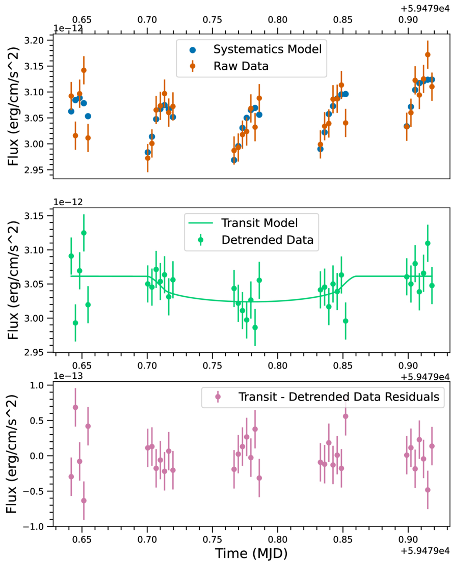
Figure 4. from Austin Baldwin et al 2026 Astron. J. 171 doi:10.3847/1538-3881/ae30e2 https://dx.doi.org/10.3847/1538-3881/ae30e2 © 2026. The Author(s). Published by the American Astronomical Society.
