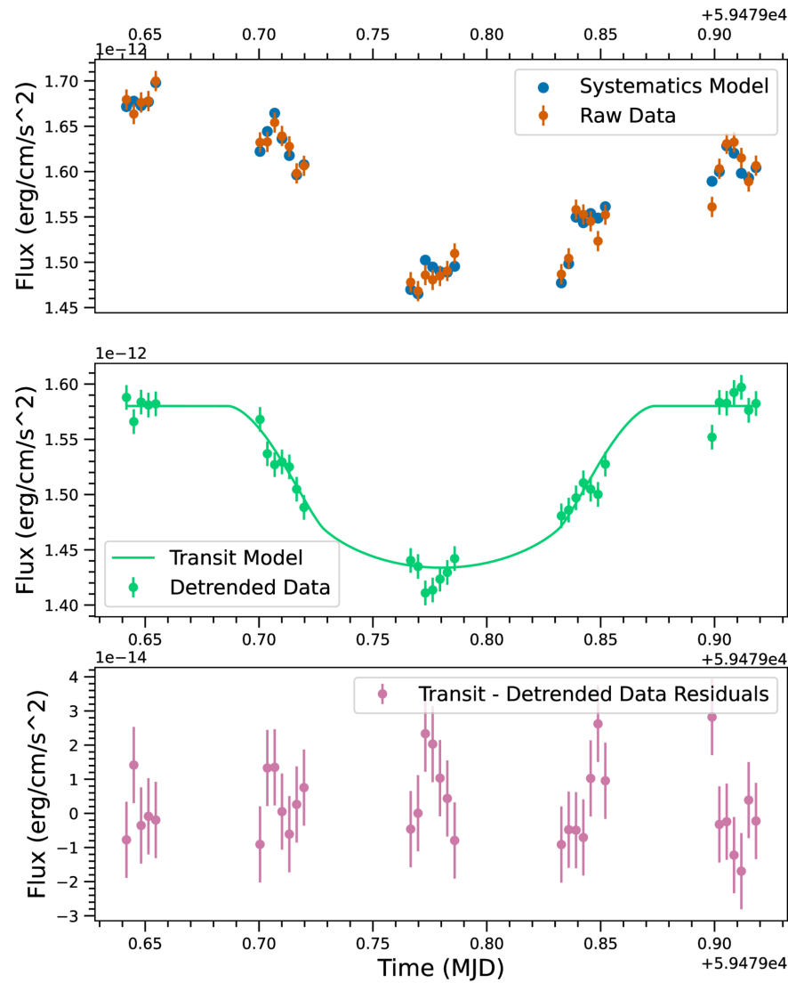
Inside Mg II (2802.4 Å)
