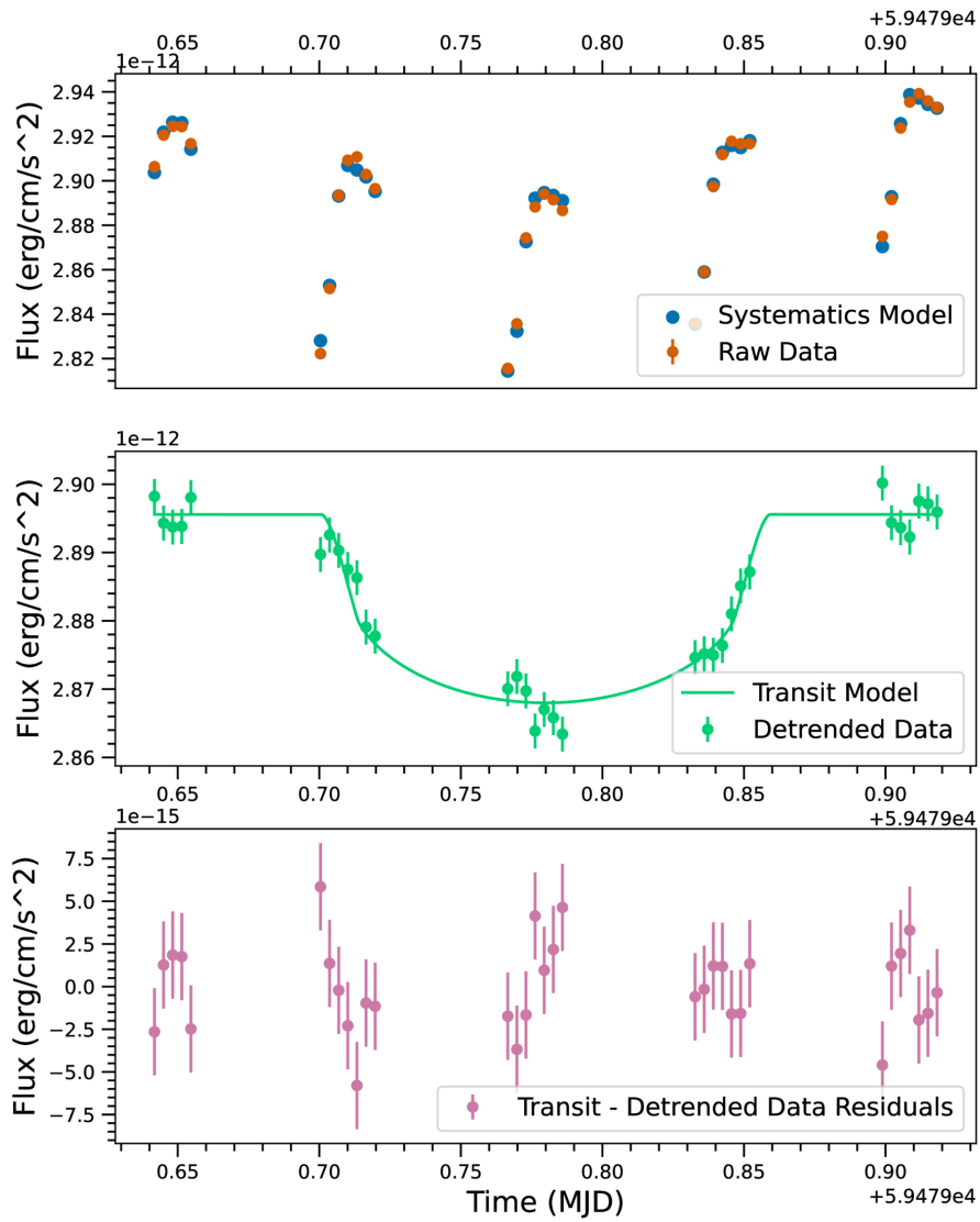
Figure 3. from Austin Baldwin et al 2026 Astron. J. 171 doi:10.3847/1538-3881/ae30e2 https://dx.doi.org/10.3847/1538-3881/ae30e2 © 2026. The Author(s). Published by the American Astronomical Society.
