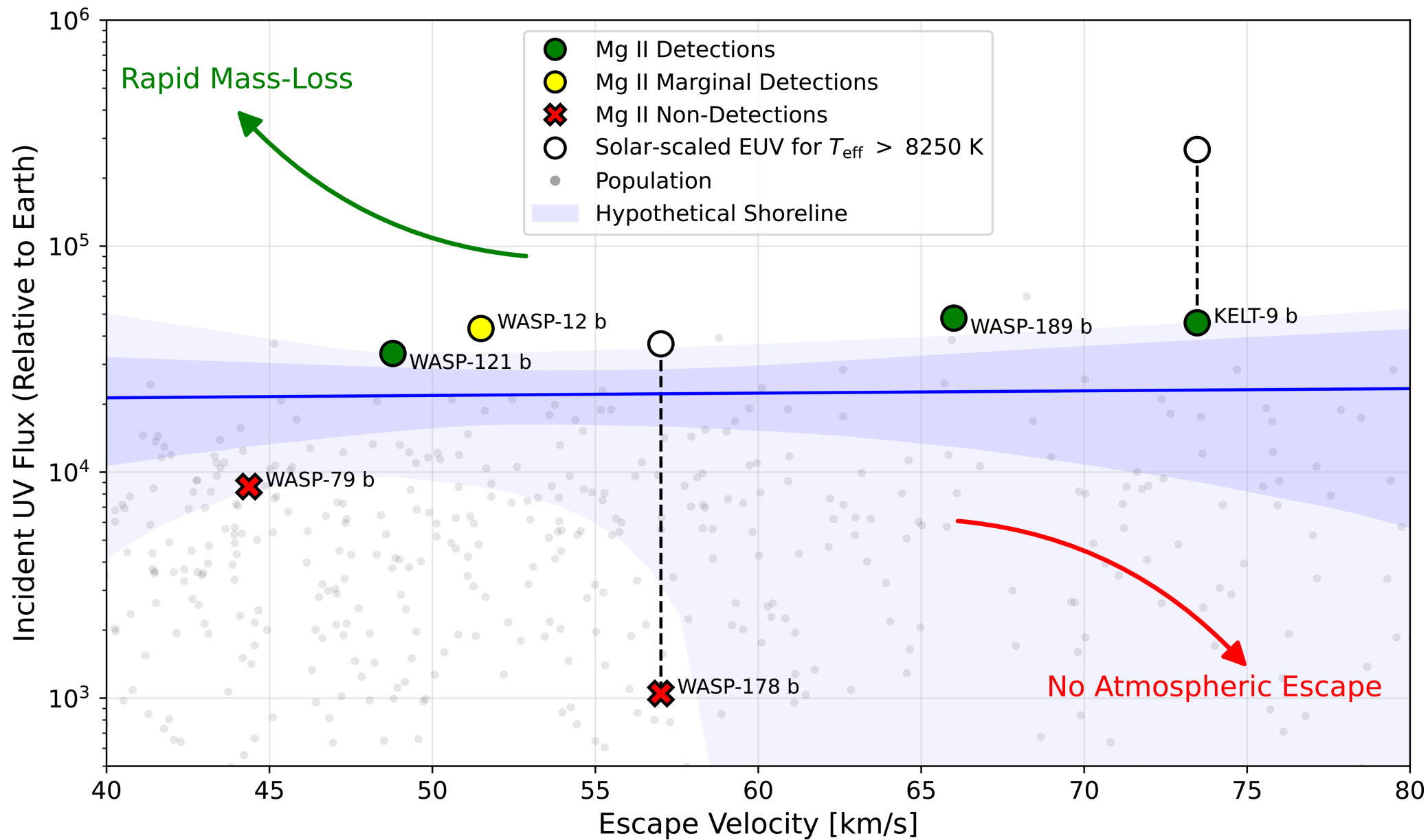
Figure 12. from Austin Baldwin et al 2026 Astron. J. 171 doi:10.3847/1538-3881/ae30e2 https://dx.doi.org/10.3847/1538-3881/ae30e2 © 2026. The Author(s). Published by the American Astronomical Society.
