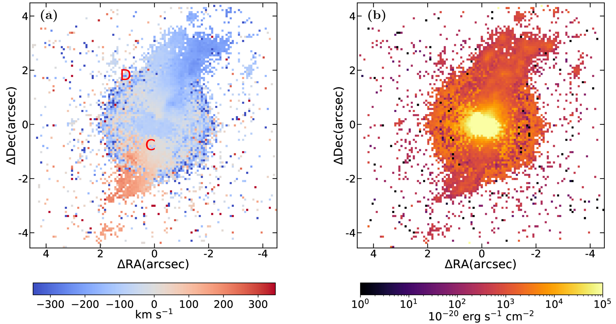
Figure 9. from Hui Guo et al 2026 Astron. J. 171 doi:10.3847/1538-3881/ae3087 https://dx.doi.org/10.3847/1538-3881/ae3087 © 2026. The Author(s). Published by the American Astronomical Society.
