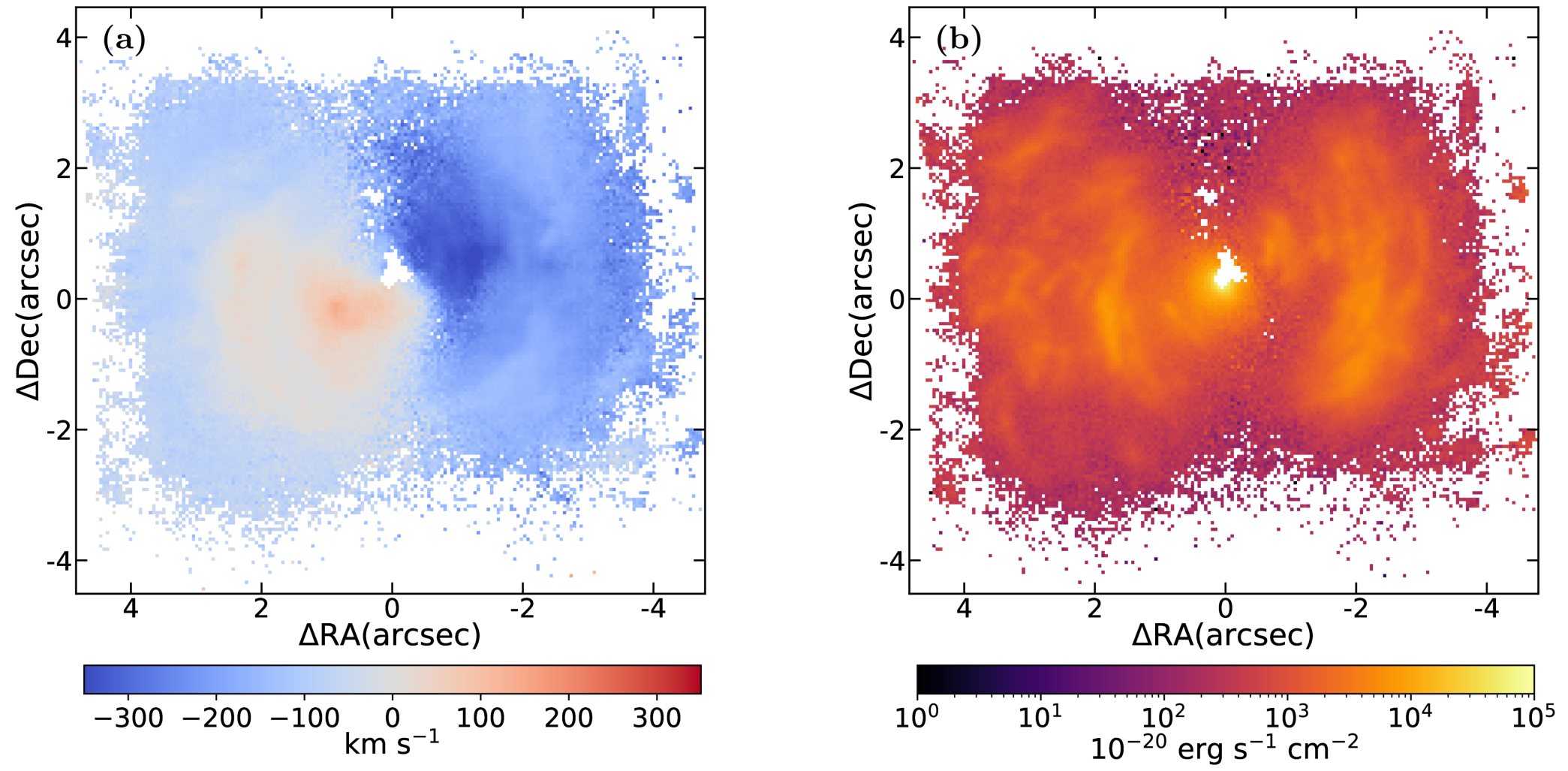
Figure 6. from Hui Guo et al 2026 Astron. J. 171 doi:10.3847/1538-3881/ae3087 https://dx.doi.org/10.3847/1538-3881/ae3087 © 2026. The Author(s). Published by the American Astronomical Society.
