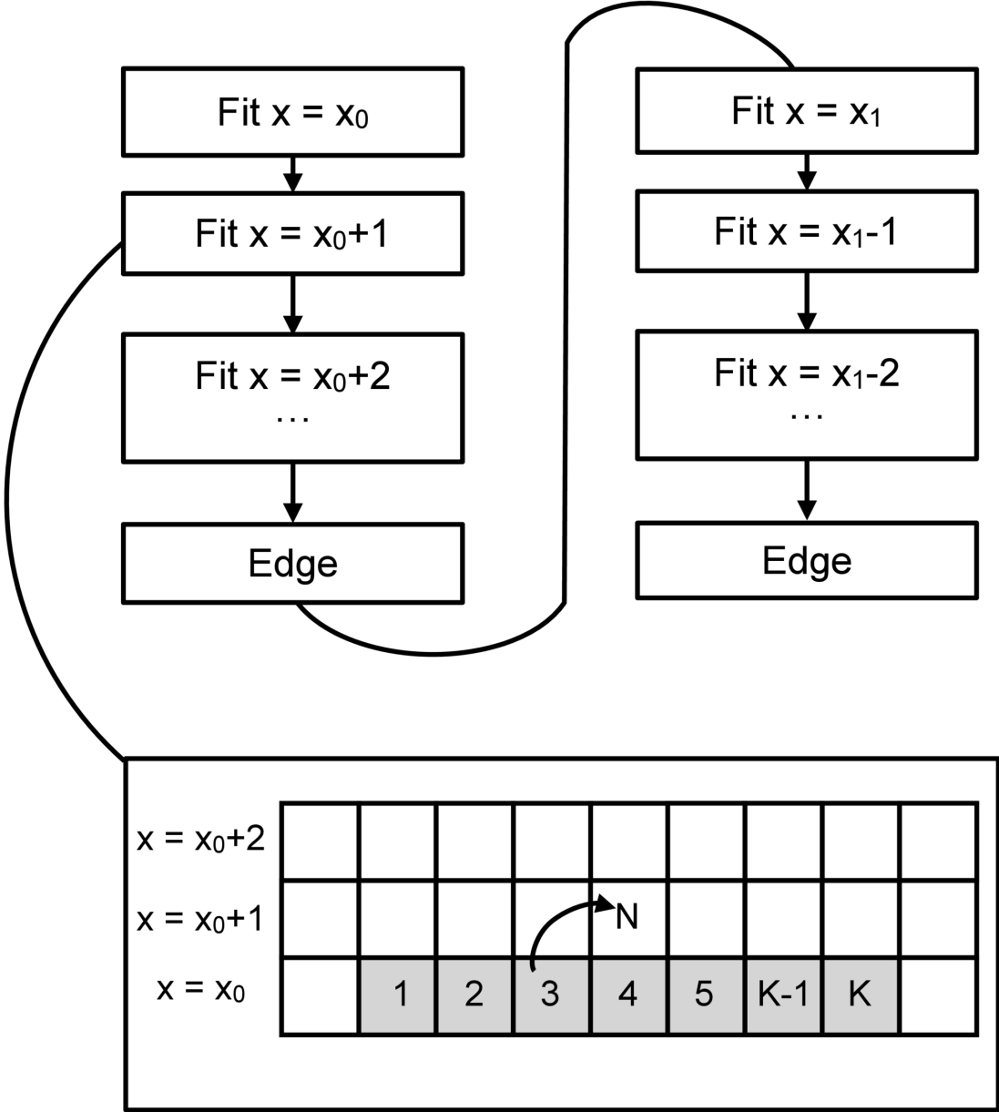
Figure 3. from Hui Guo et al 2026 Astron. J. 171 doi:10.3847/1538-3881/ae3087 https://dx.doi.org/10.3847/1538-3881/ae3087 © 2026. The Author(s). Published by the American Astronomical Society.
