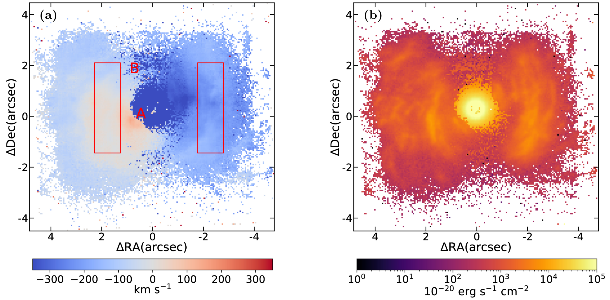
Figure 2. from Hui Guo et al 2026 Astron. J. 171 doi:10.3847/1538-3881/ae3087 https://dx.doi.org/10.3847/1538-3881/ae3087 © 2026. The Author(s). Published by the American Astronomical Society.
