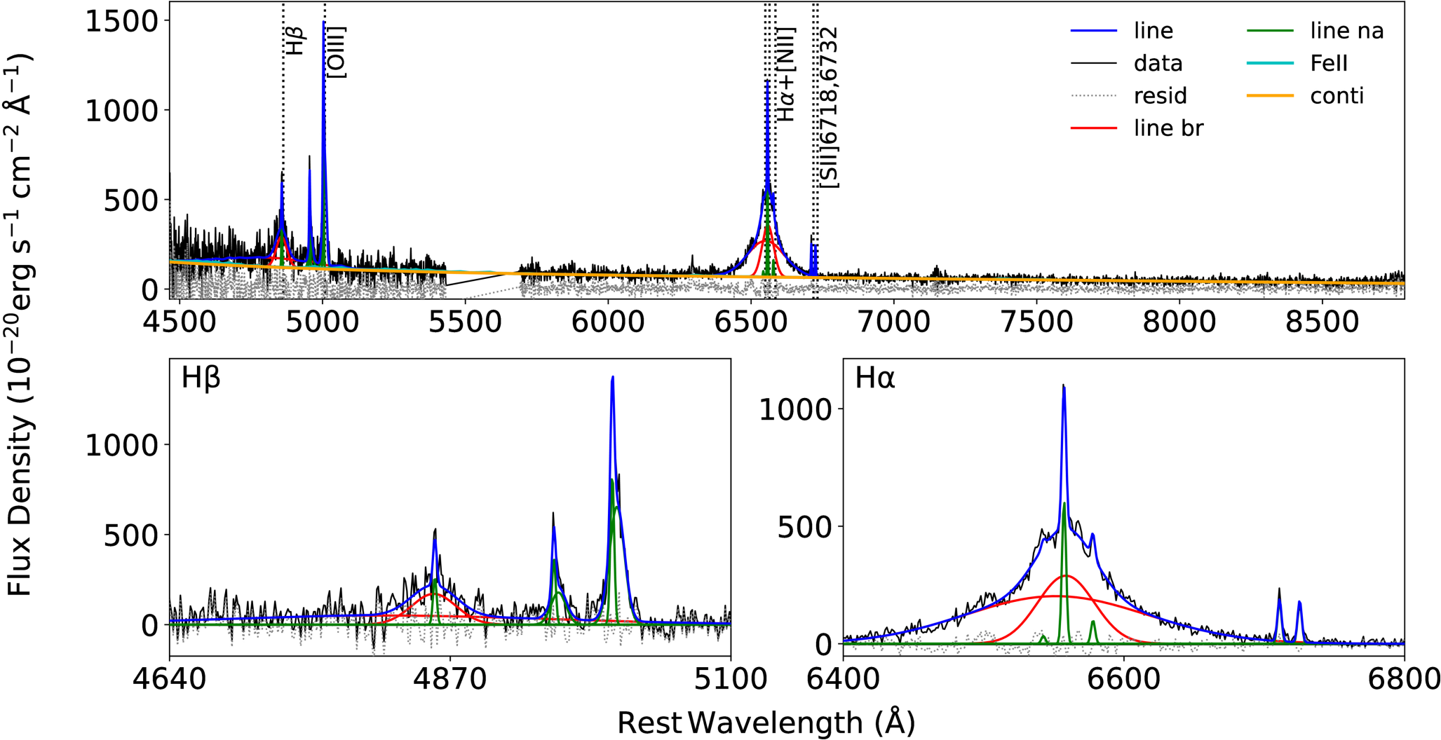
Figure 1. from Hui Guo et al 2026 Astron. J. 171 doi:10.3847/1538-3881/ae3087 https://dx.doi.org/10.3847/1538-3881/ae3087 © 2026. The Author(s). Published by the American Astronomical Society.
