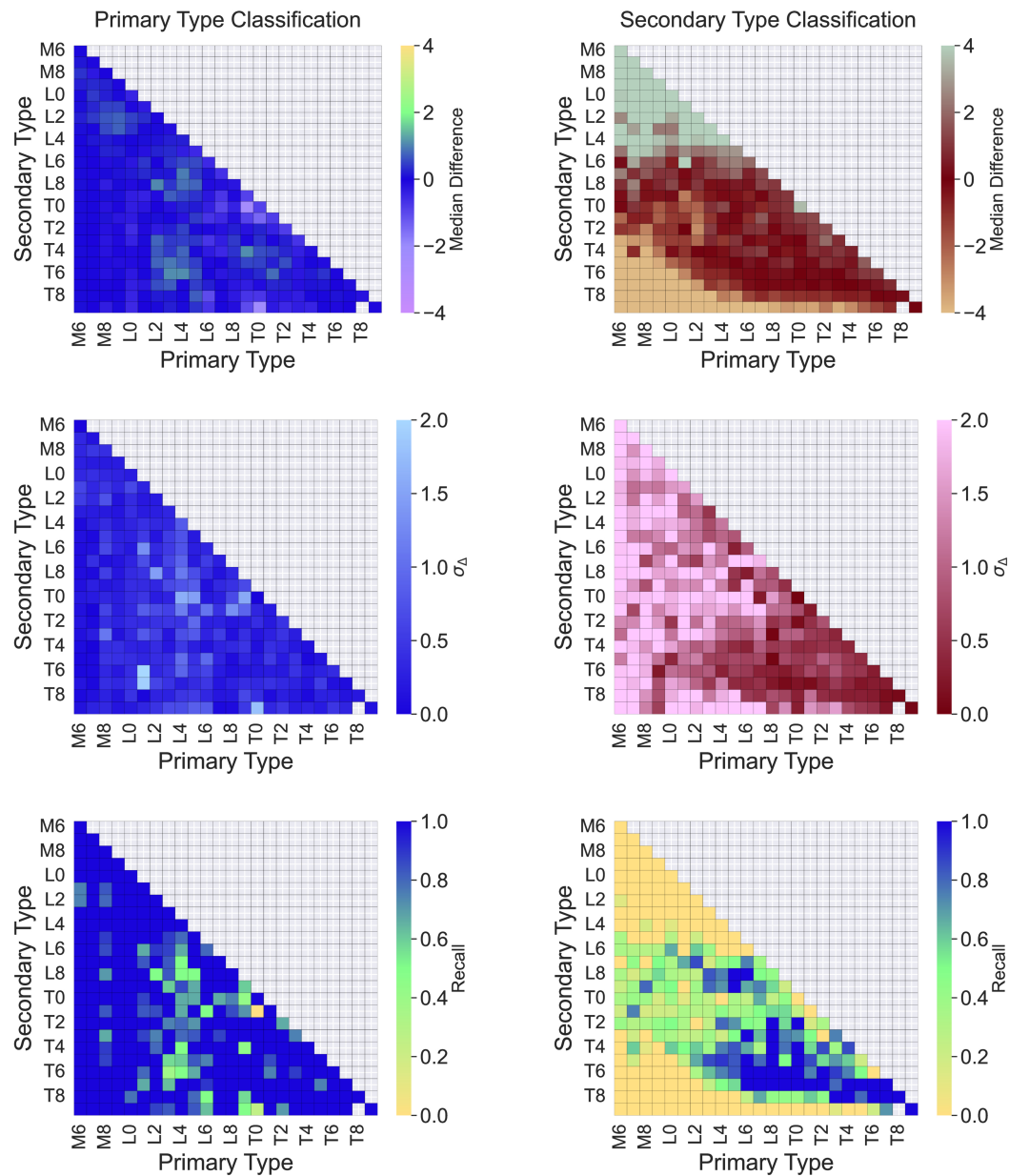
Figure 9. from Juan Diego Draxl Giannoni et al 2026 Astron. J. 171 doi:10.3847/1538-3881/ae3086 https://dx.doi.org/10.3847/1538-3881/ae3086 © 2026. The Author(s). Published by the American Astronomical Society.
