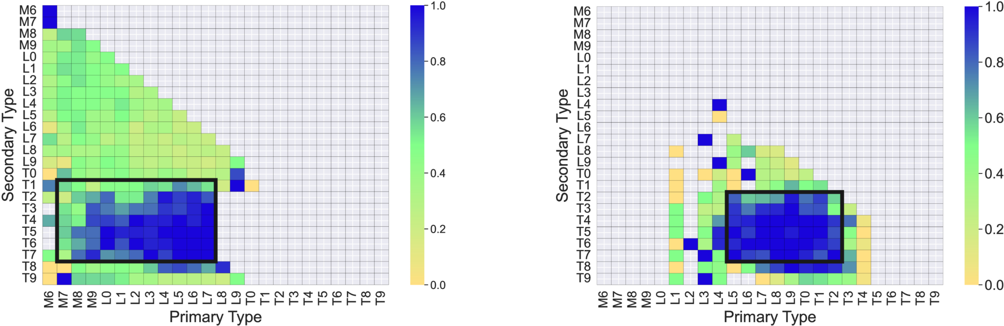
Figure 7. from Juan Diego Draxl Giannoni et al 2026 Astron. J. 171 doi:10.3847/1538-3881/ae3086 https://dx.doi.org/10.3847/1538-3881/ae3086 © 2026. The Author(s). Published by the American Astronomical Society.
