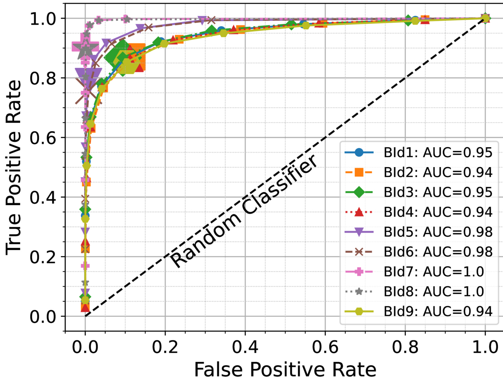
Figure 4. from Juan Diego Draxl Giannoni et al 2026 Astron. J. 171 doi:10.3847/1538-3881/ae3086 https://dx.doi.org/10.3847/1538-3881/ae3086 © 2026. The Author(s). Published by the American Astronomical Society.
