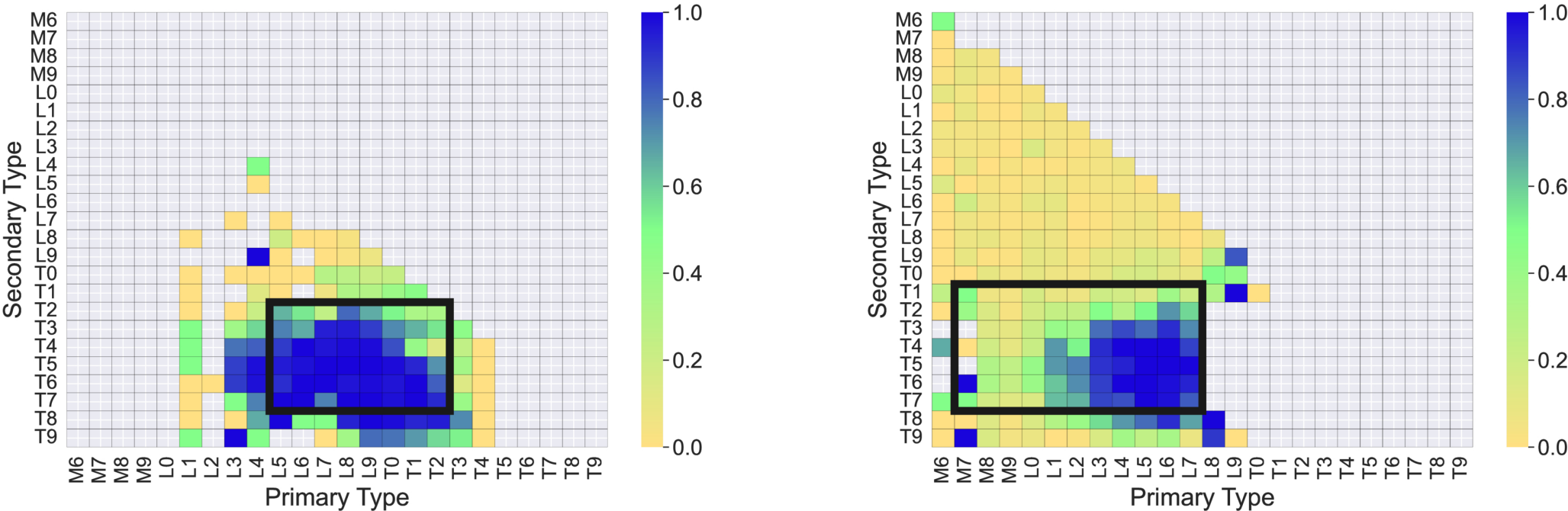
Figure 3. from Juan Diego Draxl Giannoni et al 2026 Astron. J. 171 doi:10.3847/1538-3881/ae3086 https://dx.doi.org/10.3847/1538-3881/ae3086 © 2026. The Author(s). Published by the American Astronomical Society.
