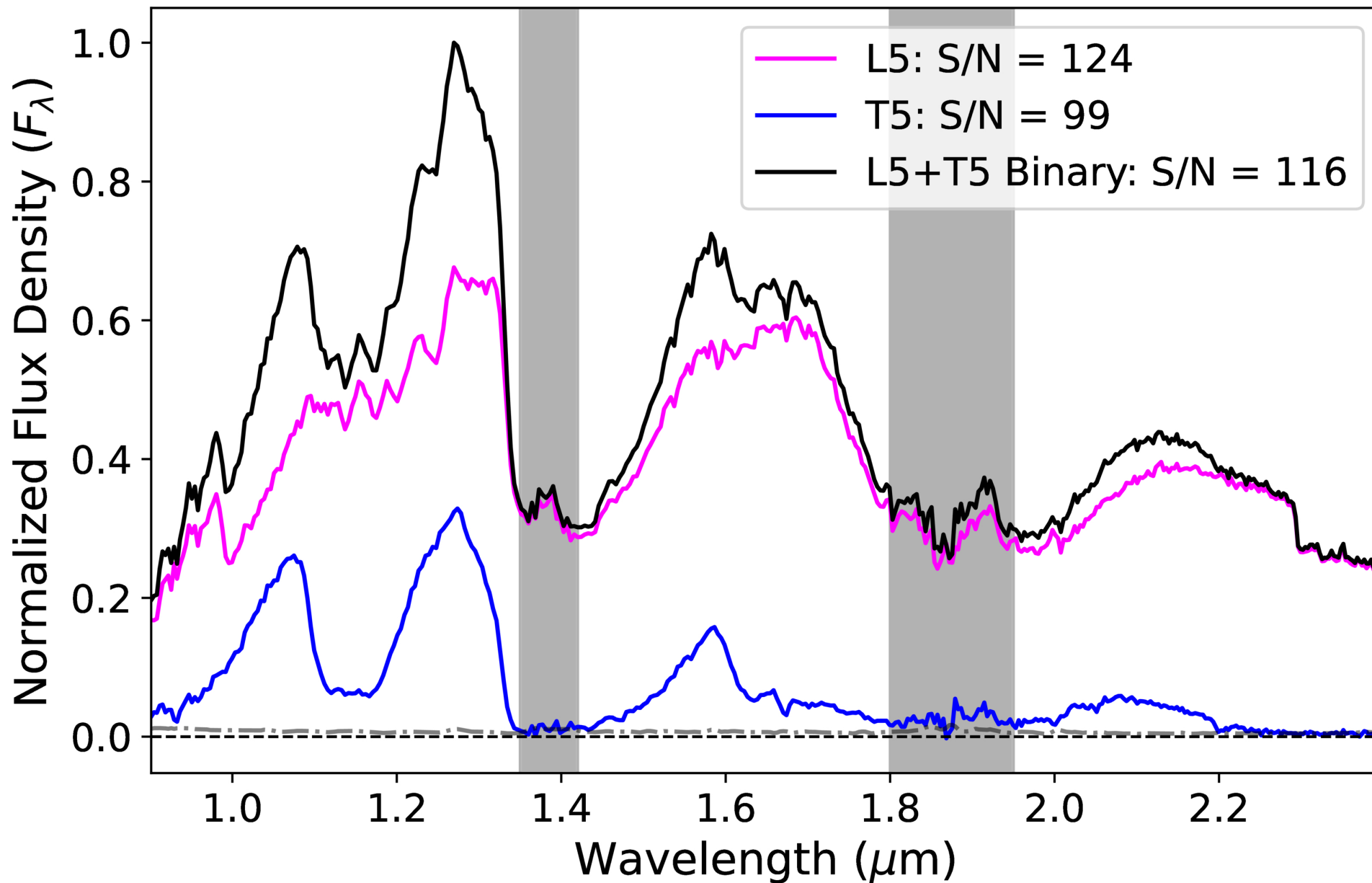
Figure 2. from Juan Diego Draxl Giannoni et al 2026 Astron. J. 171 doi:10.3847/1538-3881/ae3086 https://dx.doi.org/10.3847/1538-3881/ae3086 © 2026. The Author(s). Published by the American Astronomical Society.
