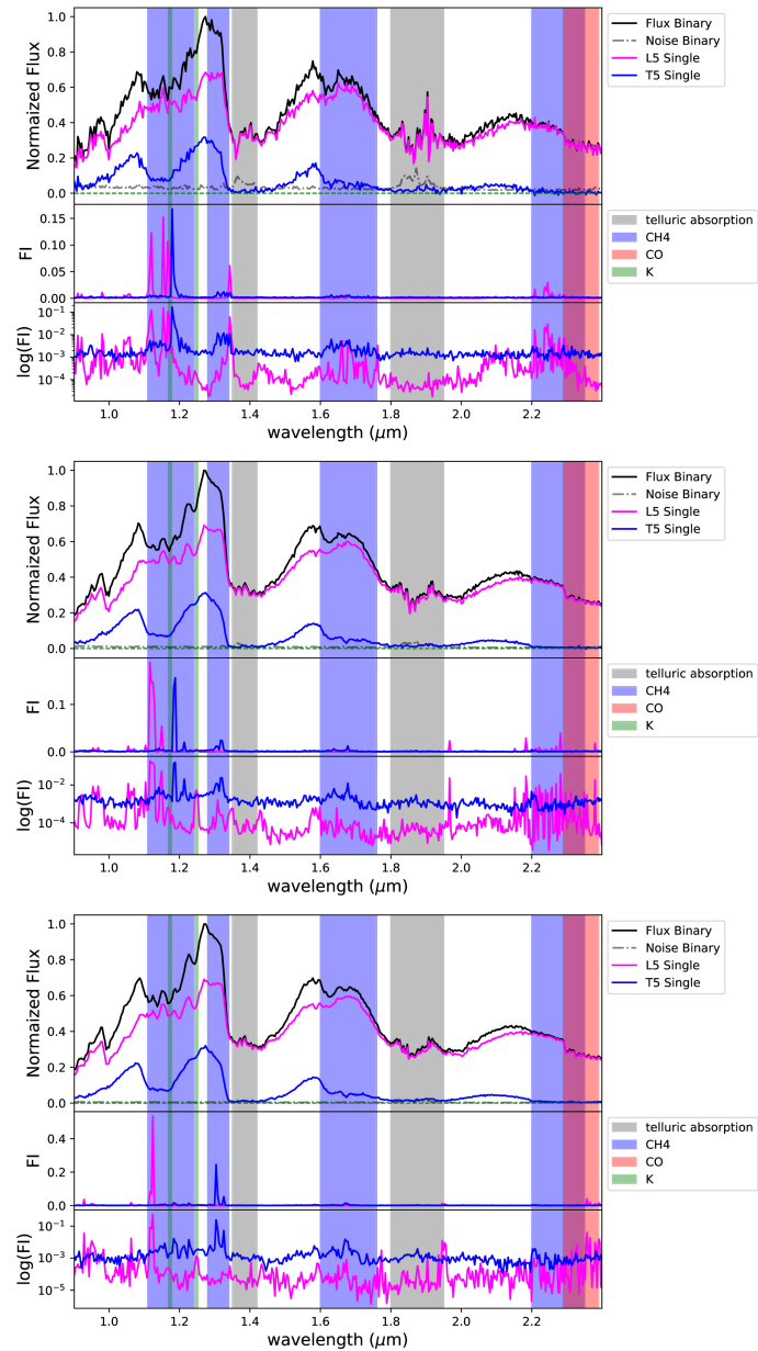
Figure 10. from Juan Diego Draxl Giannoni et al 2026 Astron. J. 171 doi:10.3847/1538-3881/ae3086 https://dx.doi.org/10.3847/1538-3881/ae3086 © 2026. The Author(s). Published by the American Astronomical Society.
