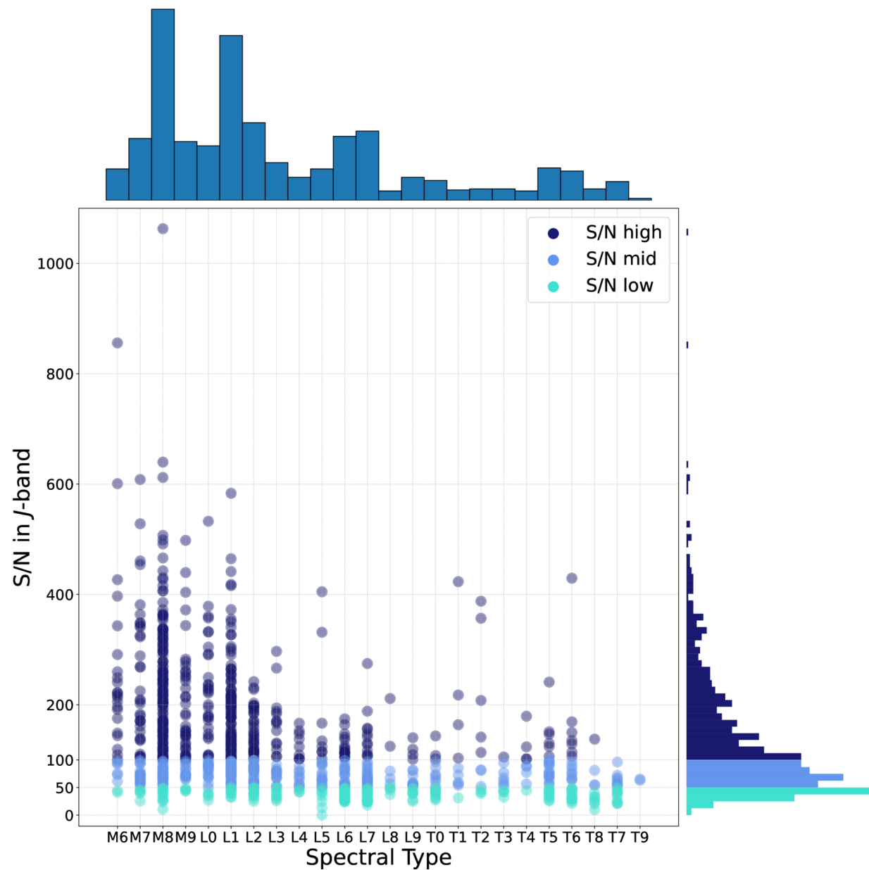
Figure 1. from Juan Diego Draxl Giannoni et al 2026 Astron. J. 171 doi:10.3847/1538-3881/ae3086 https://dx.doi.org/10.3847/1538-3881/ae3086 © 2026. The Author(s). Published by the American Astronomical Society.
