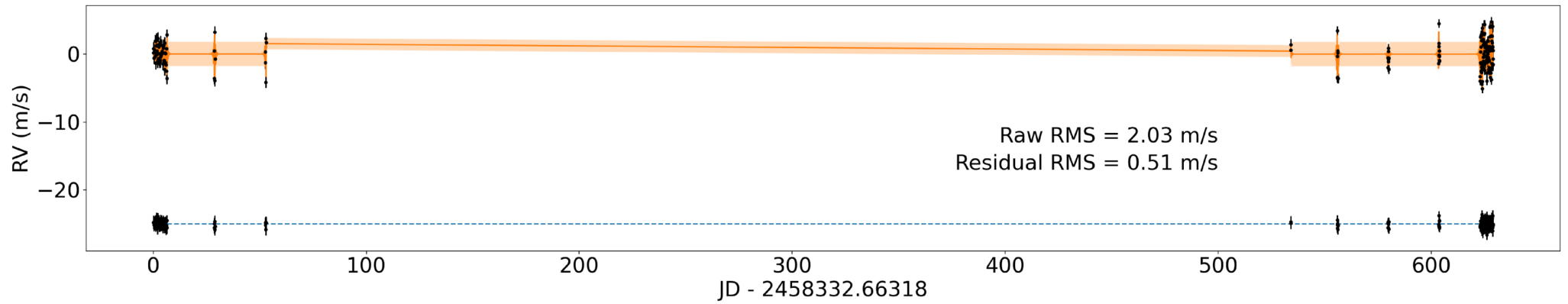
Figure 8. from Jiaxin Tang et al 2026 Astron. J. 171 doi:10.3847/1538-3881/ae307b https://dx.doi.org/10.3847/1538-3881/ae307b © 2026. The Author(s). Published by the American Astronomical Society.
