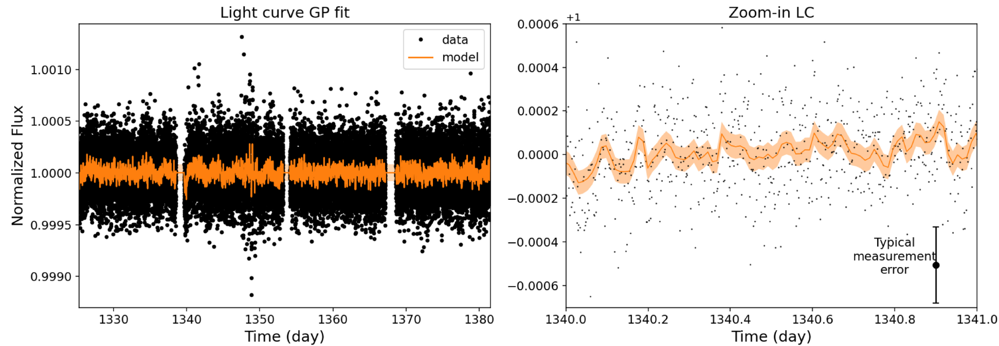
Figure 6. from Jiaxin Tang et al 2026 Astron. J. 171 doi:10.3847/1538-3881/ae307b https://dx.doi.org/10.3847/1538-3881/ae307b © 2026. The Author(s). Published by the American Astronomical Society.
