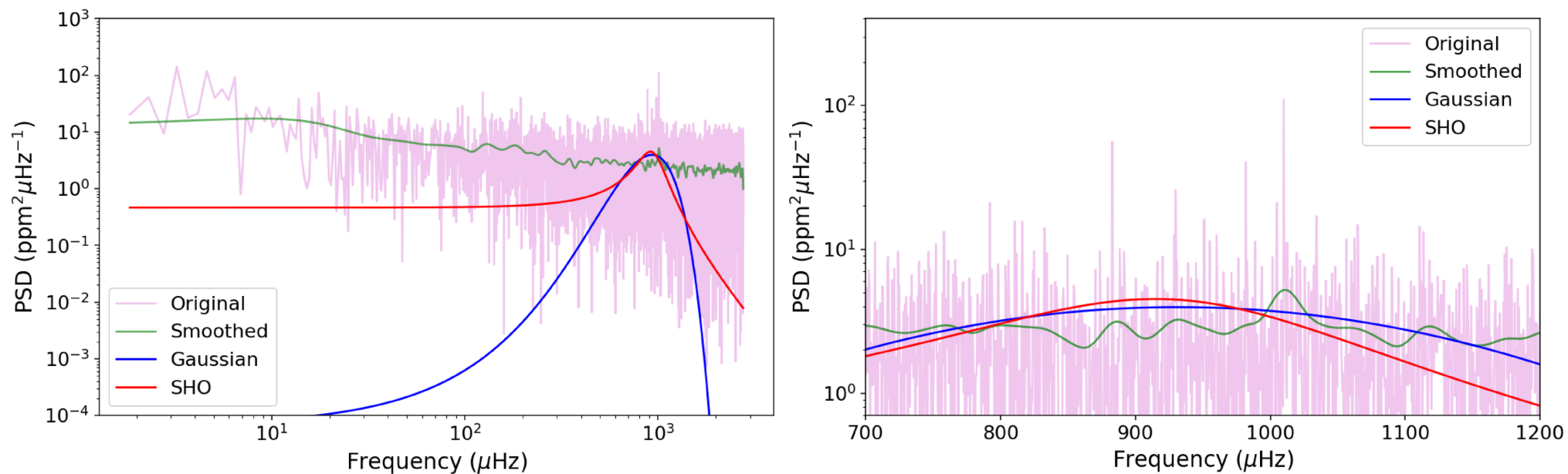
Figure 5. from Jiaxin Tang et al 2026 Astron. J. 171 doi:10.3847/1538-3881/ae307b https://dx.doi.org/10.3847/1538-3881/ae307b © 2026. The Author(s). Published by the American Astronomical Society.
