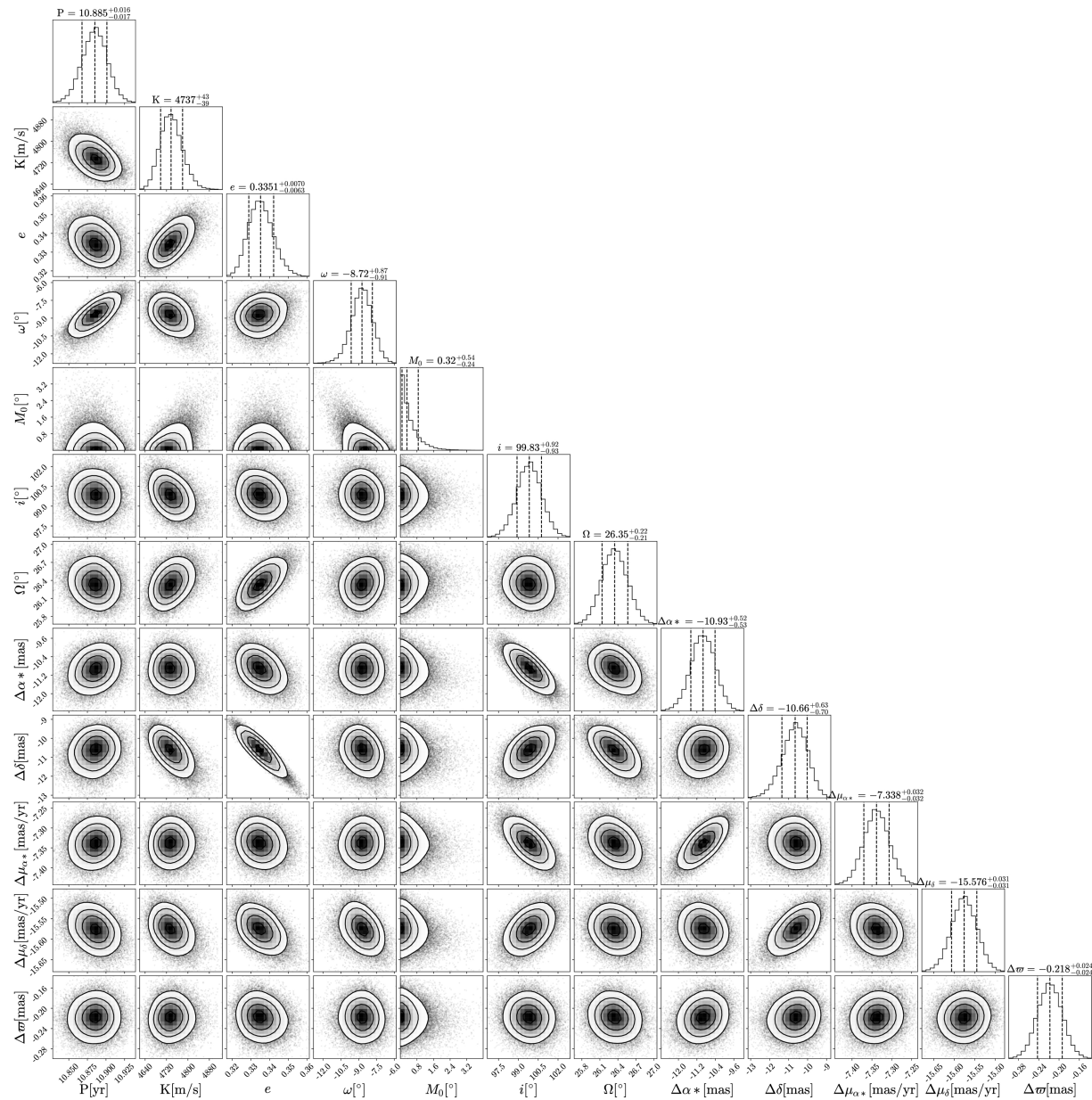
Figure 13. from Jiaxin Tang et al 2026 Astron. J. 171 doi:10.3847/1538-3881/ae307b https://dx.doi.org/10.3847/1538-3881/ae307b © 2026. The Author(s). Published by the American Astronomical Society.
