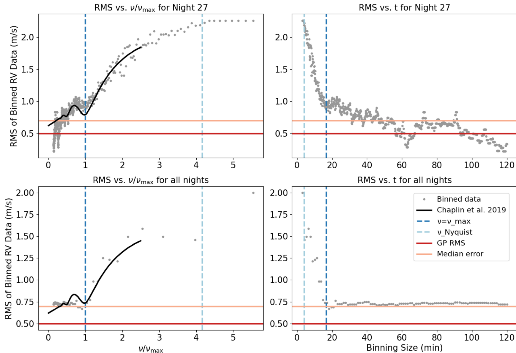
Figure 12. from Jiaxin Tang et al 2026 Astron. J. 171 doi:10.3847/1538-3881/ae307b https://dx.doi.org/10.3847/1538-3881/ae307b © 2026. The Author(s). Published by the American Astronomical Society.
