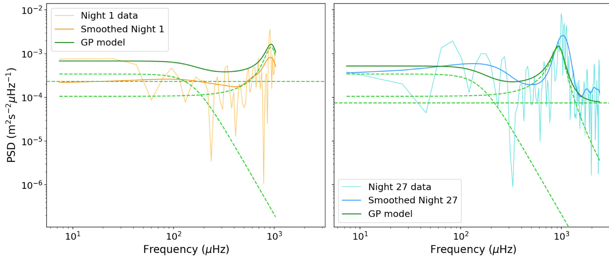
Figure 10. from Jiaxin Tang et al 2026 Astron. J. 171 doi:10.3847/1538-3881/ae307b https://dx.doi.org/10.3847/1538-3881/ae307b © 2026. The Author(s). Published by the American Astronomical Society.
