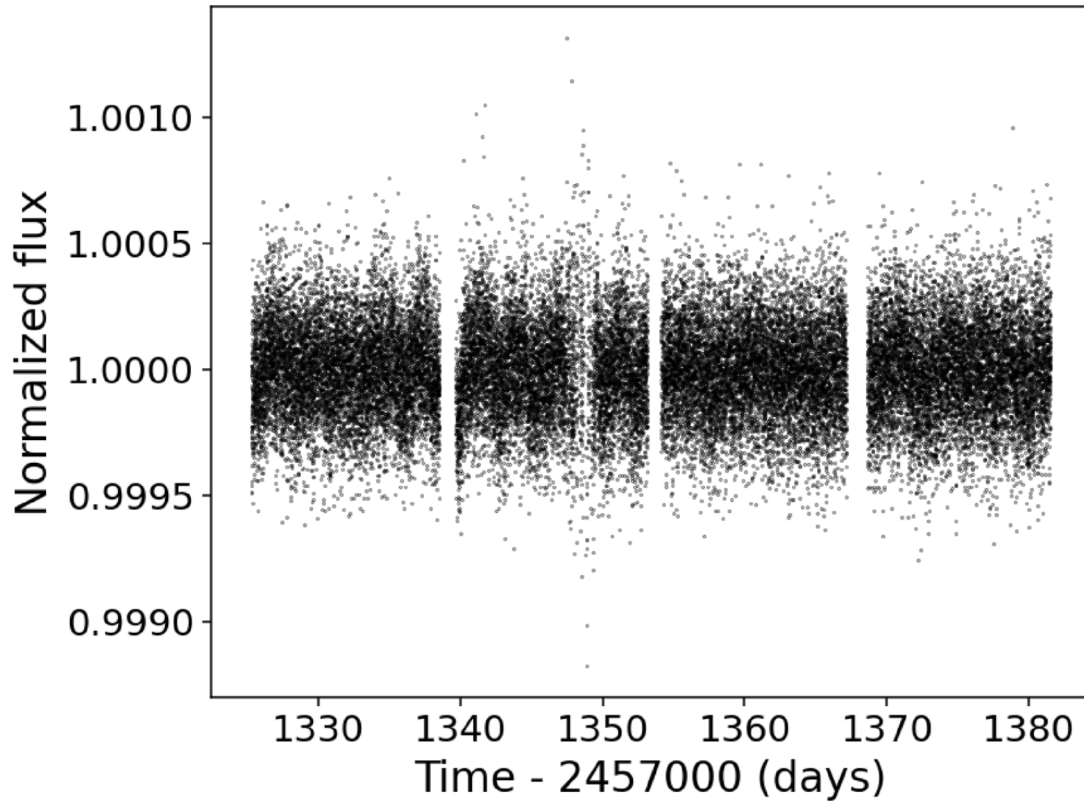
Figure 1. from Jiaxin Tang et al 2026 Astron. J. 171 doi:10.3847/1538-3881/ae307b https://dx.doi.org/10.3847/1538-3881/ae307b © 2026. The Author(s). Published by the American Astronomical Society.
