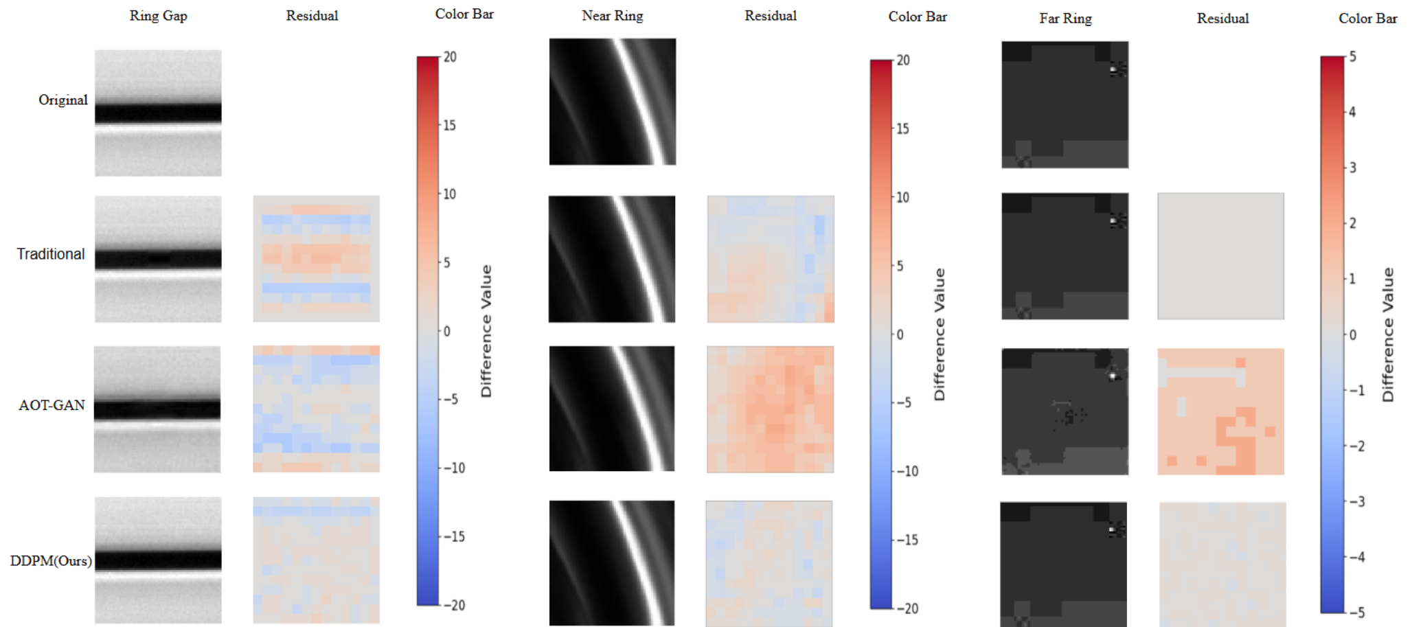
Figure 4. from Yongxin Chen et al 2026 Astron. J. 171 doi:10.3847/1538-3881/ae3001 https://dx.doi.org/10.3847/1538-3881/ae3001 © 2026. The Author(s). Published by the American Astronomical Society.
