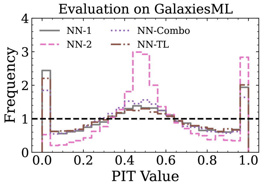
Figure 8. from Jonathan Soriano et al 2026 Astron. J. 171 doi:10.3847/1538-3881/ae2ffe https://dx.doi.org/10.3847/1538-3881/ae2ffe © 2026. The Author(s). Published by the American Astronomical Society.
