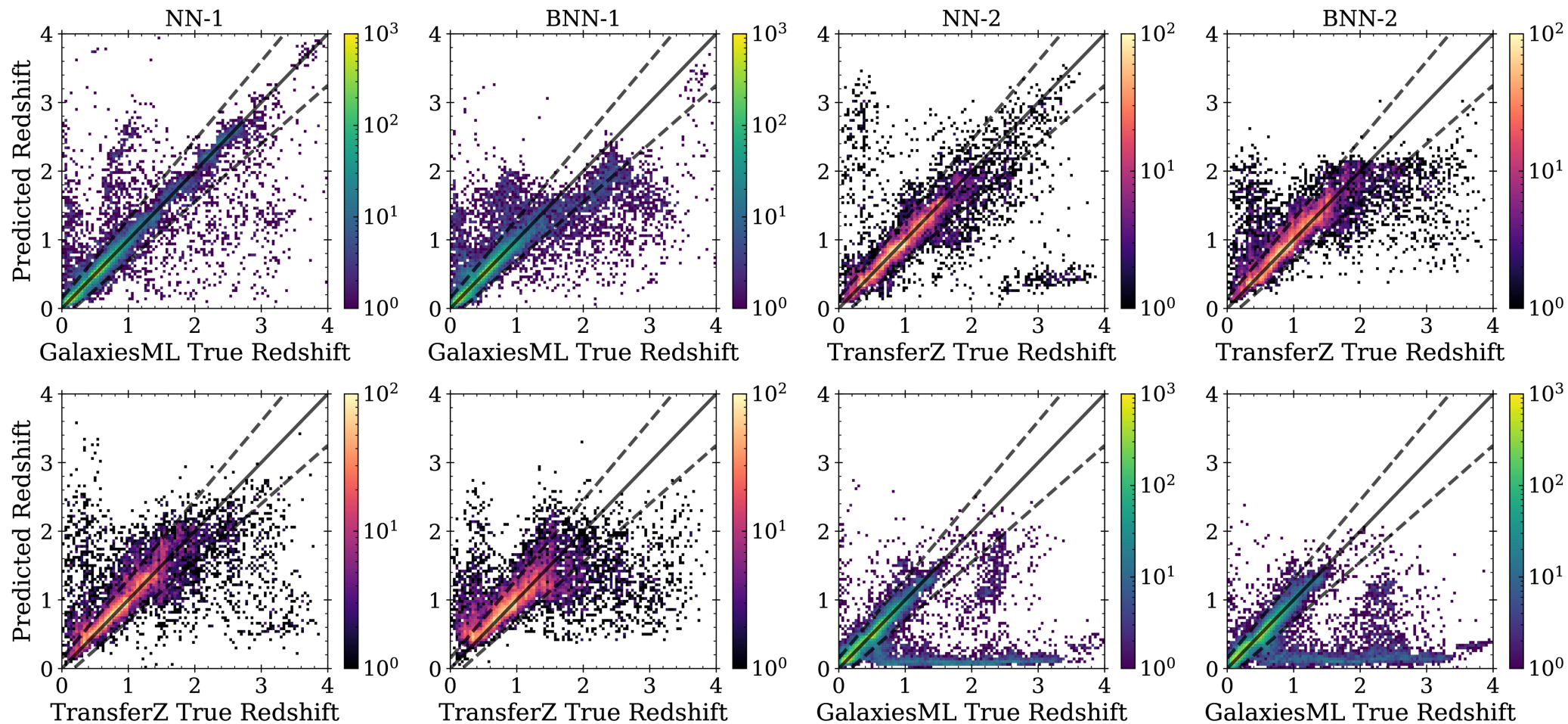
Figure 4. from Jonathan Soriano et al 2026 Astron. J. 171 doi:10.3847/1538-3881/ae2ffe https://dx.doi.org/10.3847/1538-3881/ae2ffe © 2026. The Author(s). Published by the American Astronomical Society.
