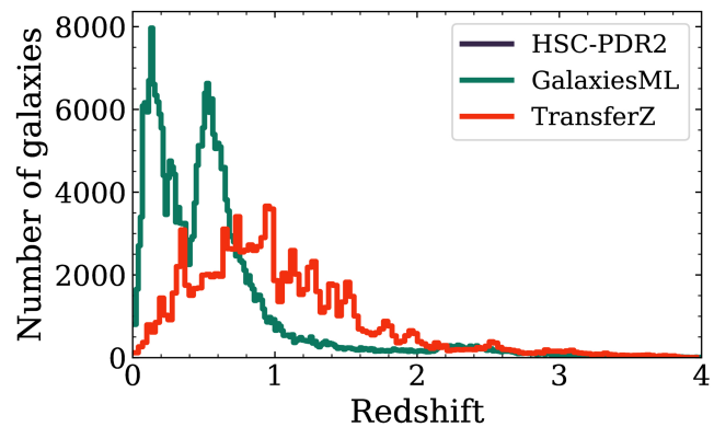
Figure 2. from Jonathan Soriano et al 2026 Astron. J. 171 doi:10.3847/1538-3881/ae2ffe https://dx.doi.org/10.3847/1538-3881/ae2ffe © 2026. The Author(s). Published by the American Astronomical Society.
