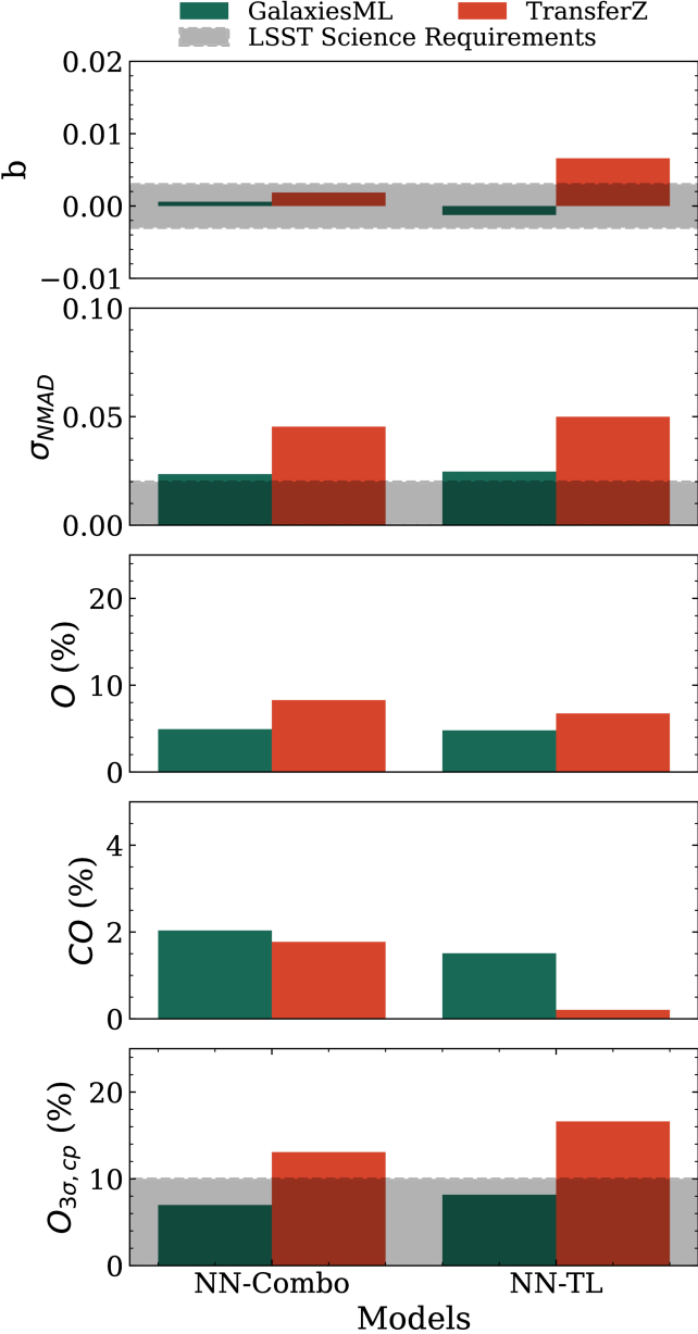
Figure 11. from Jonathan Soriano et al 2026 Astron. J. 171 doi:10.3847/1538-3881/ae2ffe https://dx.doi.org/10.3847/1538-3881/ae2ffe © 2026. The Author(s). Published by the American Astronomical Society.
