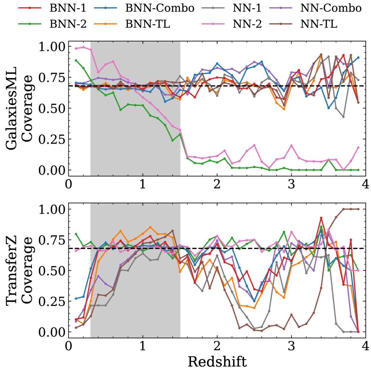
Figure 10. from Jonathan Soriano et al 2026 Astron. J. 171 doi:10.3847/1538-3881/ae2ffe https://dx.doi.org/10.3847/1538-3881/ae2ffe
