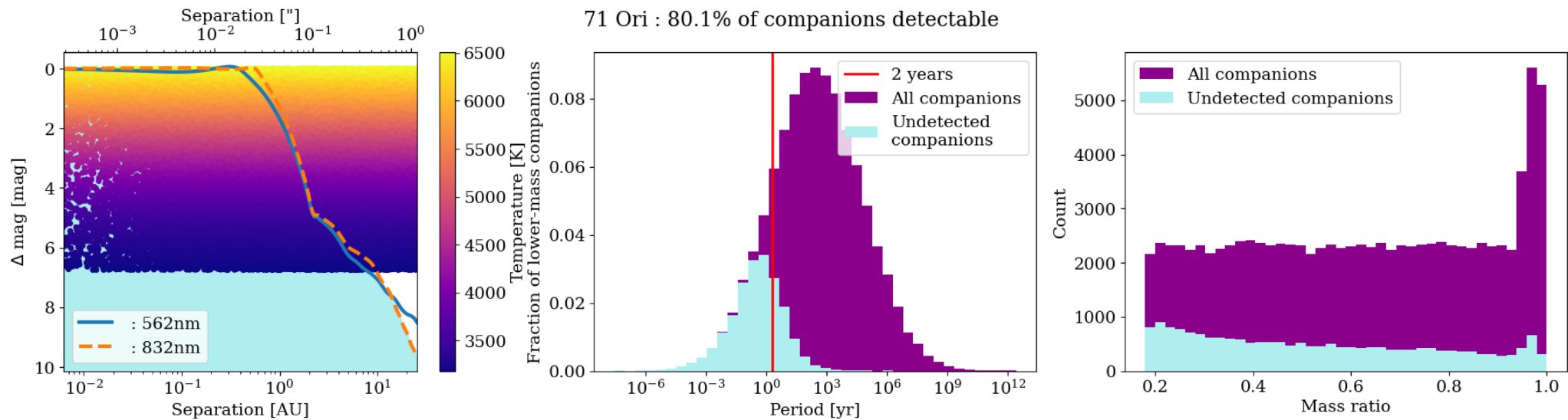
Figure 8. Missing companion analysis for the 80 targets in this study. from Zachary D. Hartman et al 2026 Astron. J. 171 doi:10.3847/1538-3881/ae2fe7 https://dx.doi.org/10.3847/1538-3881/ae2fe7 © 2026. The Author(s). Published by the American Astronomical Society.
