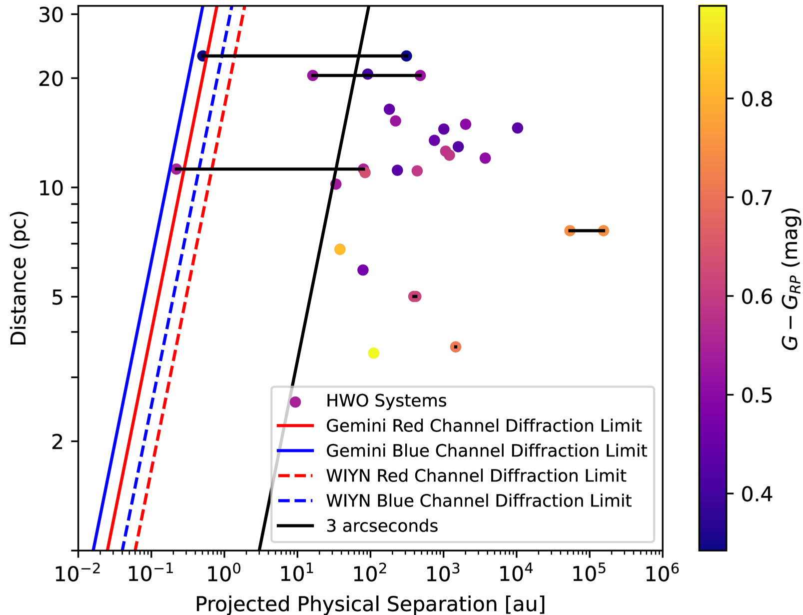
Figure 5. from Zachary D. Hartman et al 2026 Astron. J. 171 doi:10.3847/1538-3881/ae2fe7 https://dx.doi.org/10.3847/1538-3881/ae2fe7 © 2026. The Author(s). Published by the American Astronomical Society.
