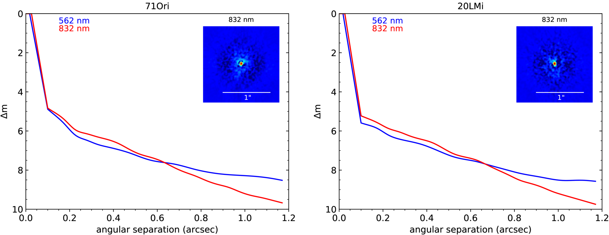
Figure 2. from Zachary D. Hartman et al 2026 Astron. J. 171 doi:10.3847/1538-3881/ae2fe7 https://dx.doi.org/10.3847/1538-3881/ae2fe7 © 2026. The Author(s). Published by the American Astronomical Society.
